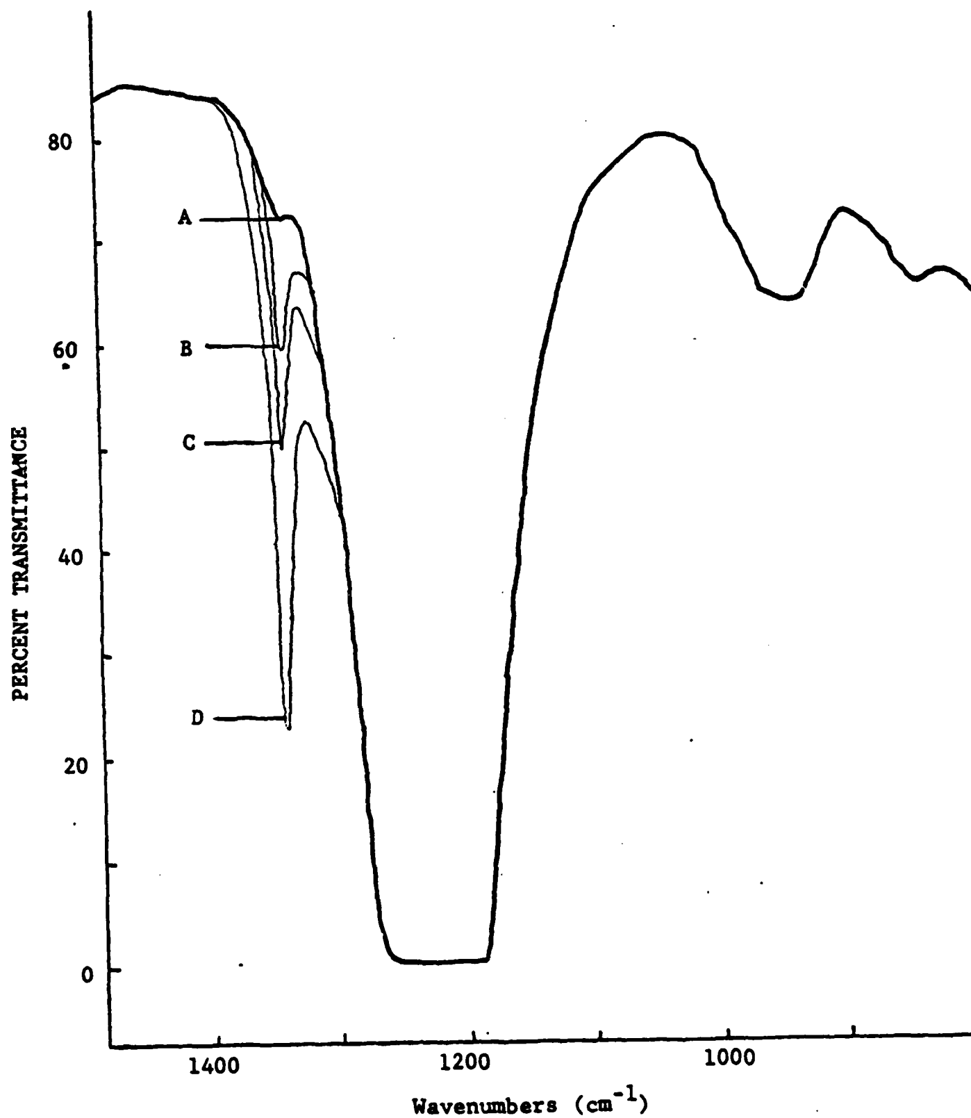
Figure 17: Infrared Spectra of 1.8M \text{LiAlCl}_4/\text{SOCl}_2 with Increasing Amounts of \text{SO}_2
