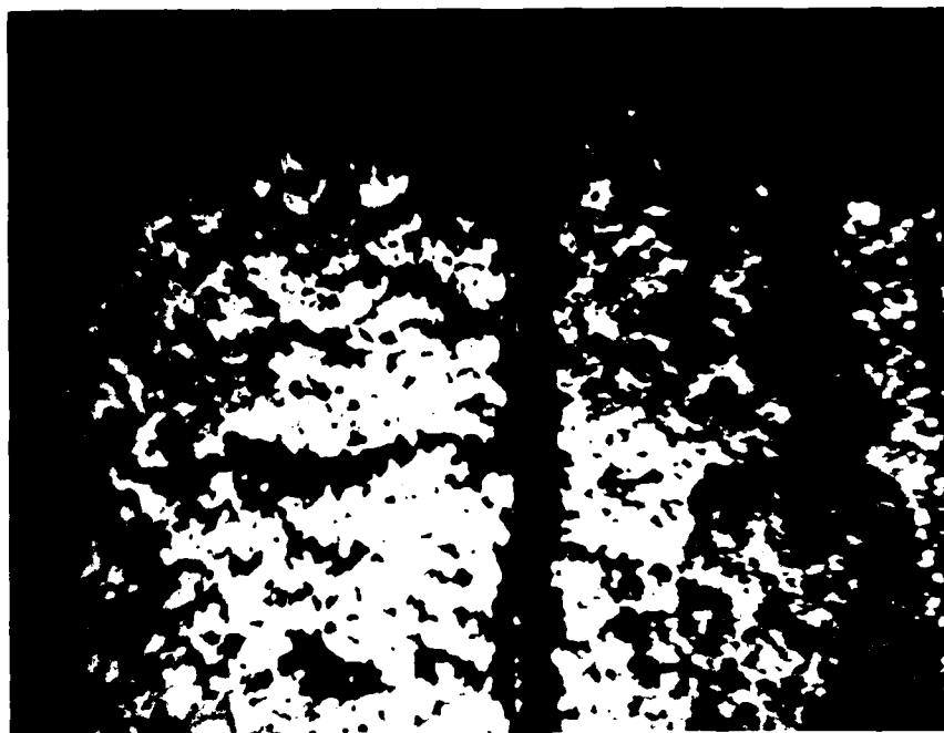
Figure 48: The Electrode of Cell 5 After 54 mAh/cm 2 of charging at 20 mA/cm 2 , 7X Magnification.
