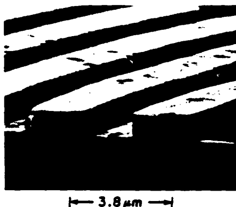
Figure 4. Scanning electron micrograph of nickel die used to emboss PVDF gratings.
