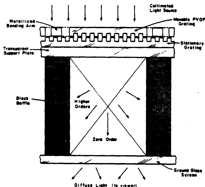
Figure 3. Schematic cross section of a pixel element of the flat panel display.
