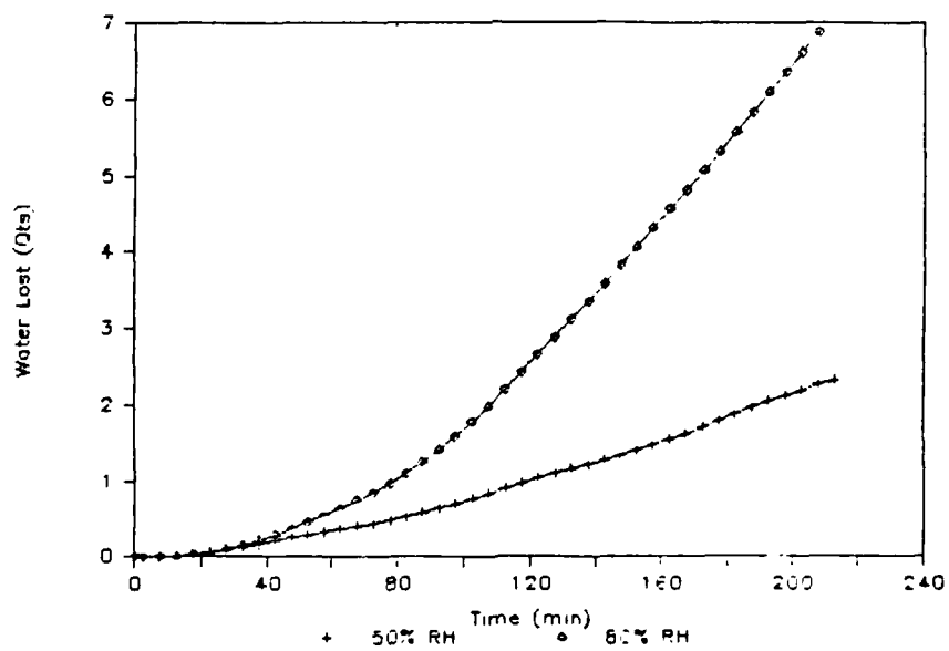
Figure 4-29: Water Lost vs. Time. Low Work, 33^{\circ}\text{C} , [40-30 Cycle]
