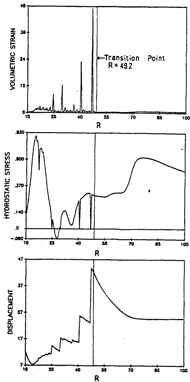
Figure 8c. Results of spherical wave problem with viscous damping for three meshes.
