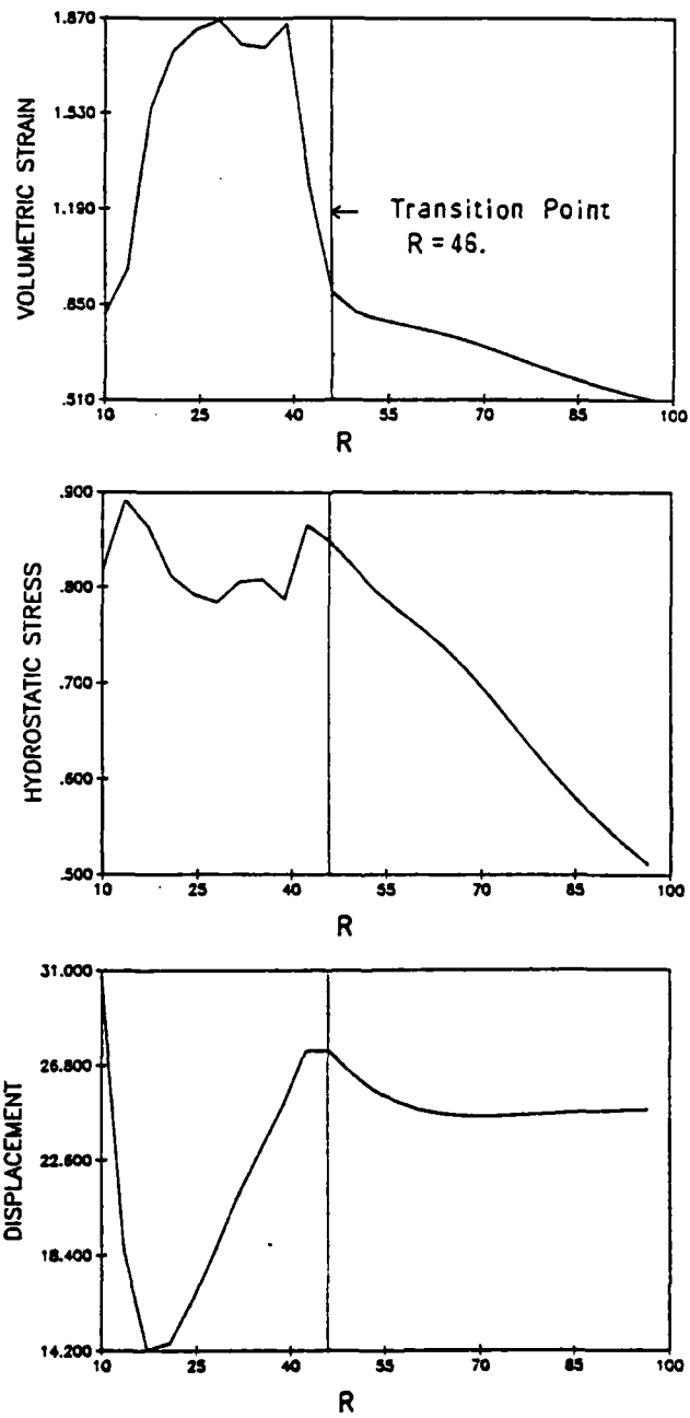
Figure 8a. Results of spherical wave problem with viscous damping for three meshes.
