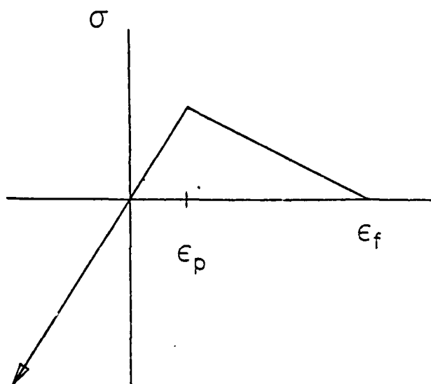
Figure 2. Stress-strain law with strain-softening and nomenclature.
