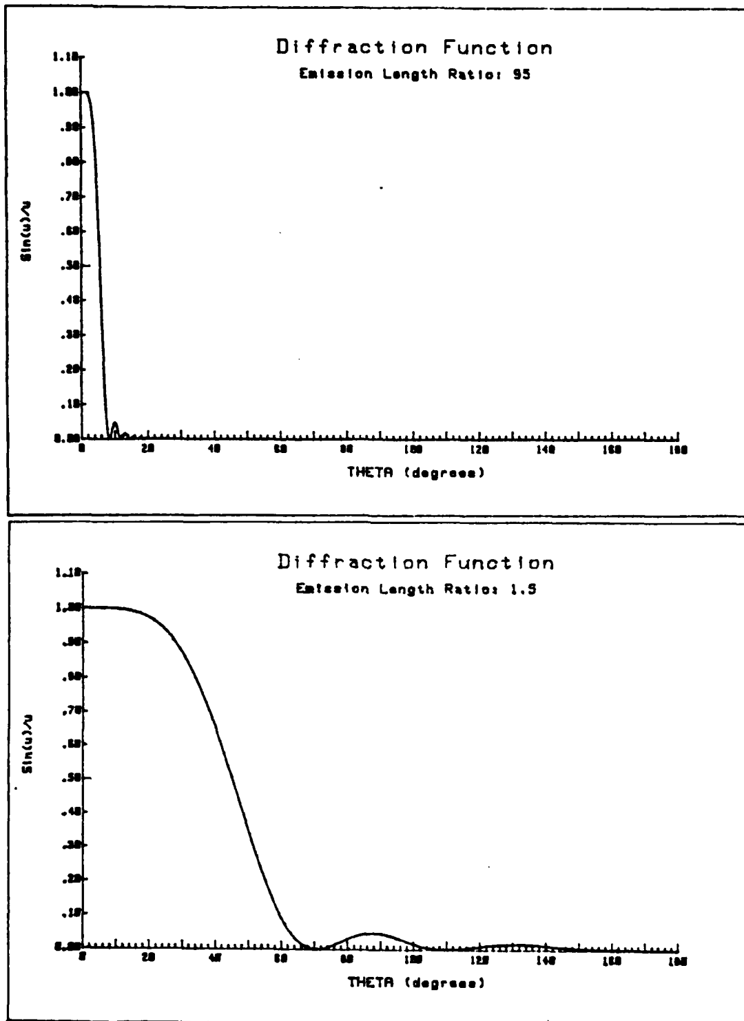
Figure 1.2 Effects of the Emission Length Ratio
