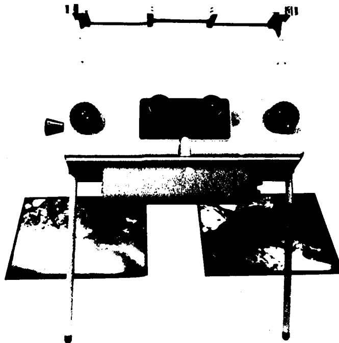
Figure 4. Old Delft scanning stereoscope
