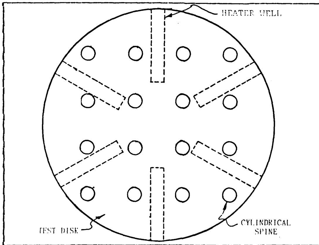
Figure 2.3 Sketch of Front View of Test Disk
