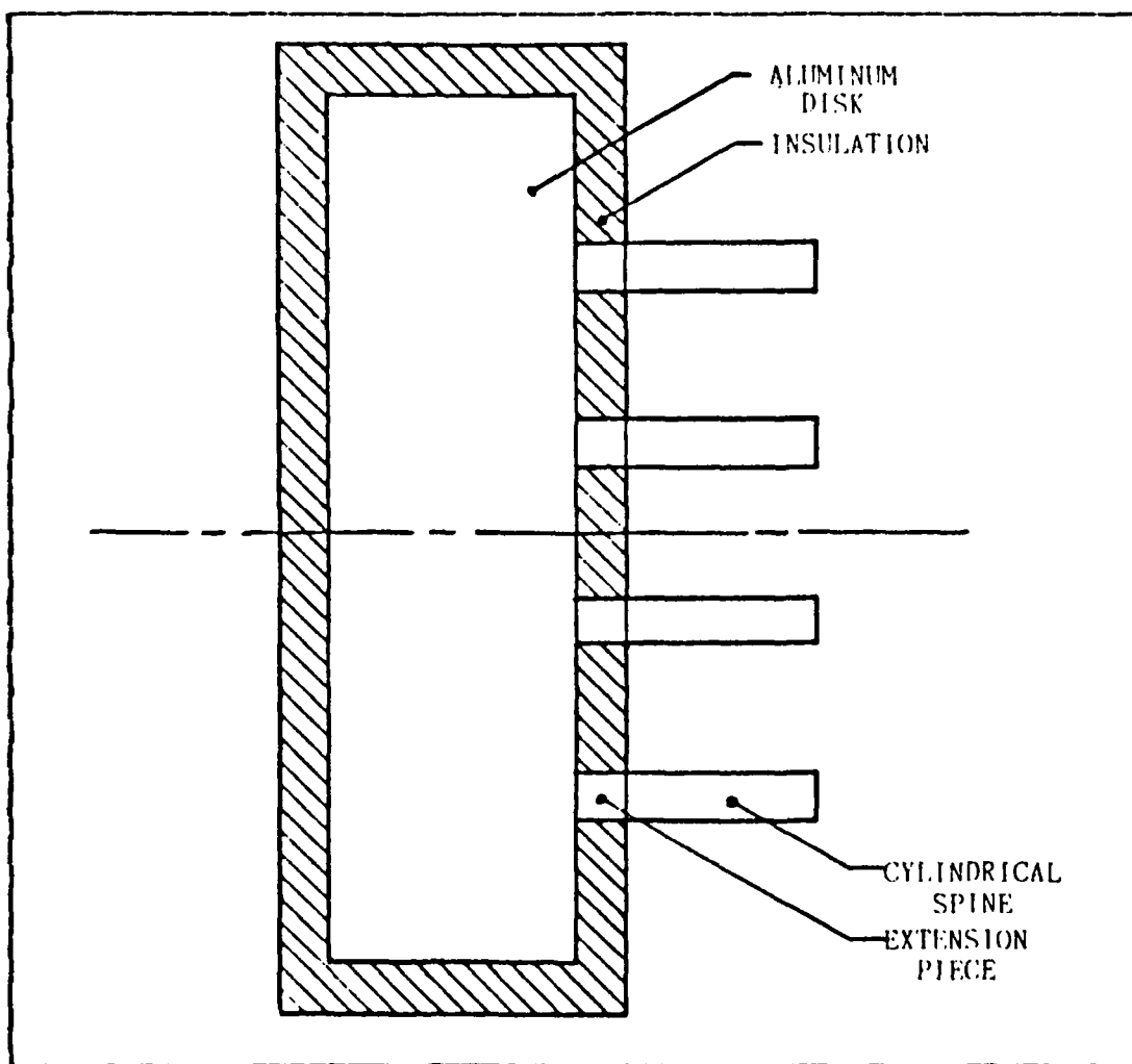
Figure 2.4 Test Disk and Spine Arrangement
