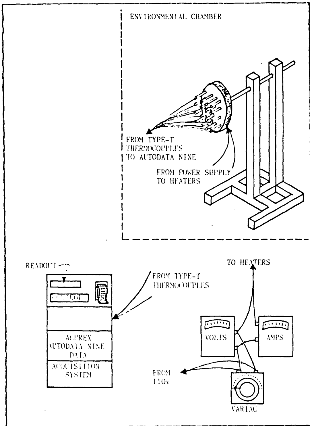
Figure 2.1 Sketch of the Test Apparatus and Configuration
