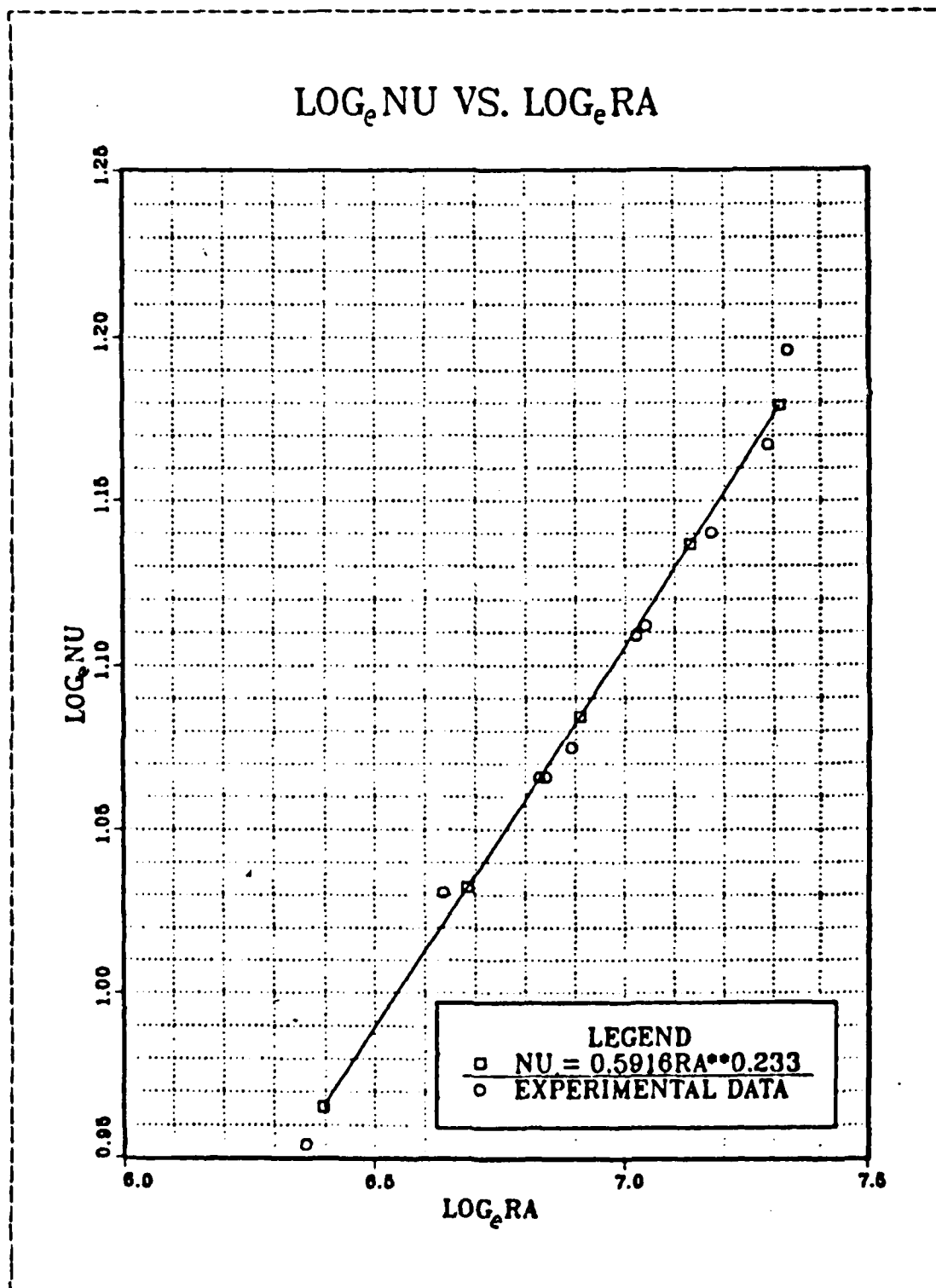
Figure E.1 \log_e \text{Nu} vs. \log_e \text{Ra} (0 degrees roll).
