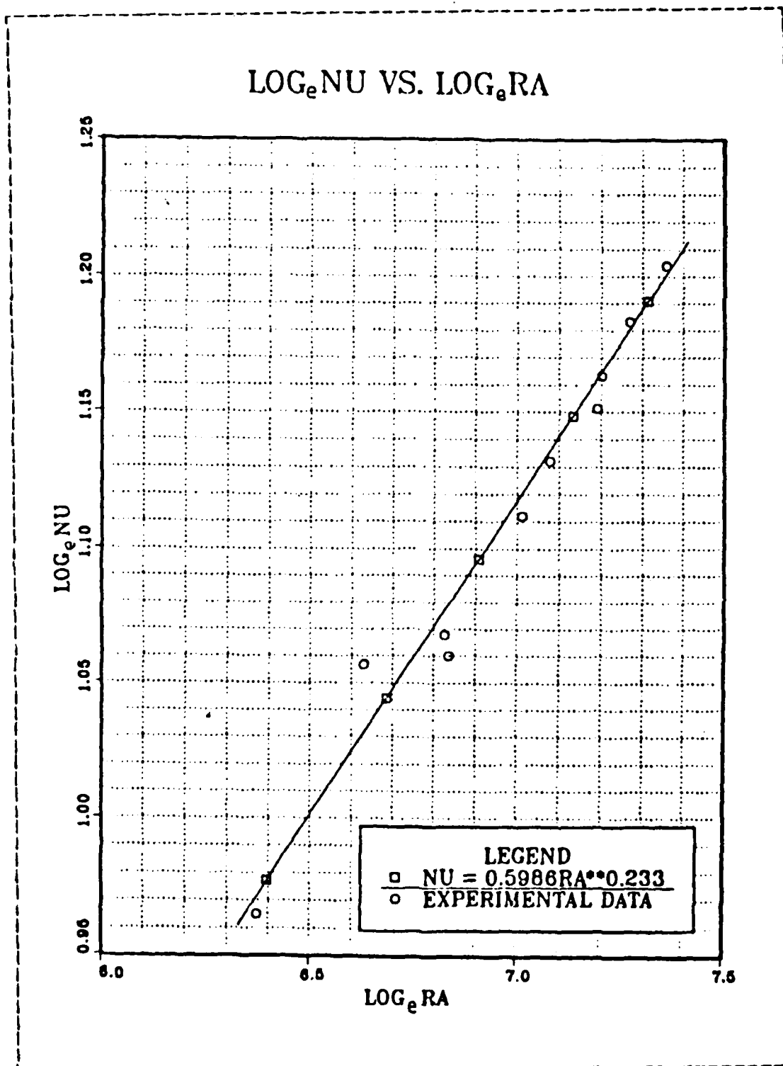
Figure B.2 \log_e \text{NU} vs. \log_e \text{Ra} (10 degrees roll).
