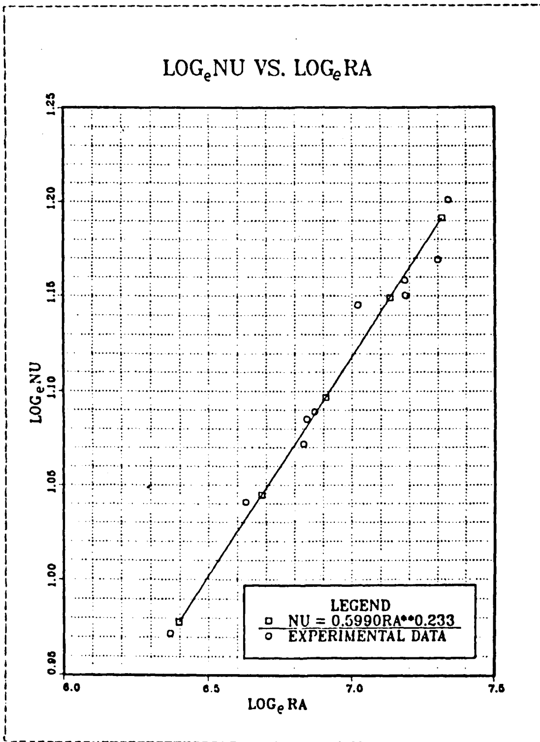
Figure B.4 \log_e \text{Nu} vs. \log_e \text{Ra} (30 degrees roll).
