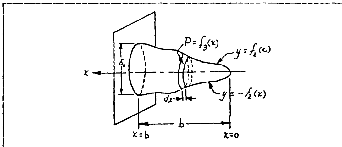
Figure A.1 Spine of Arbitrary Profile
