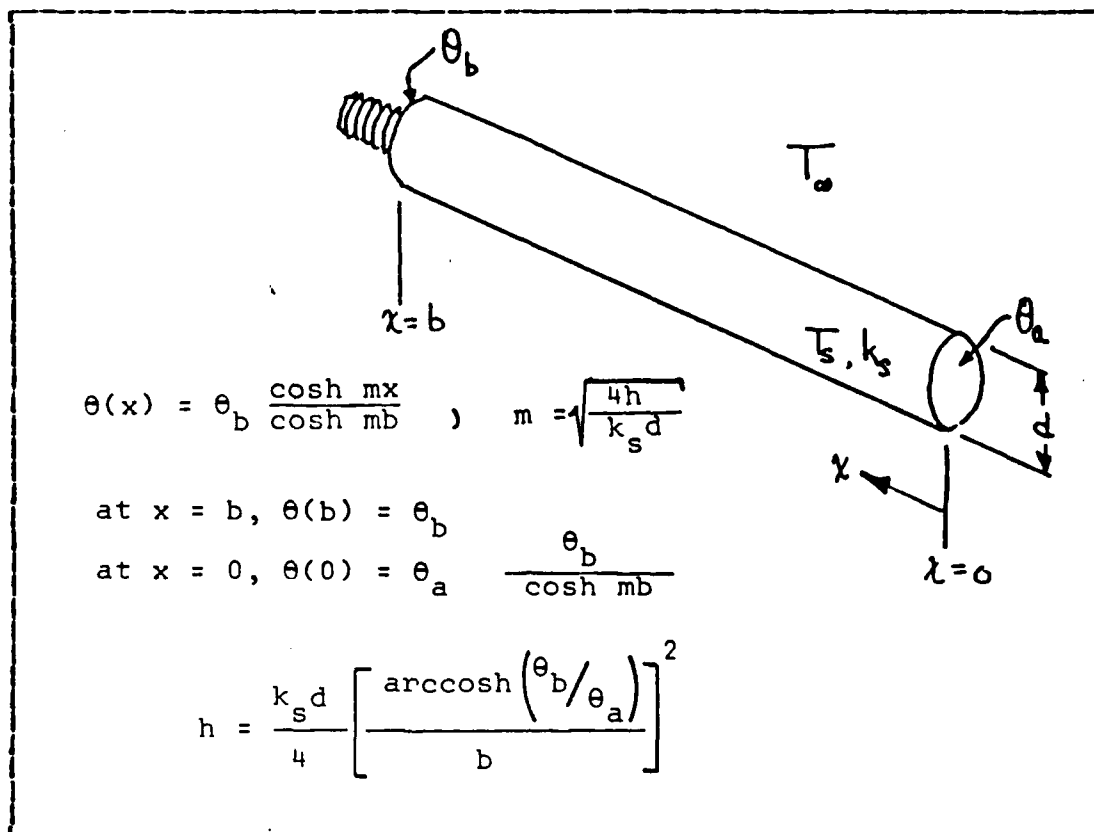
Figure 1.1 A Relation for the Heat Transfer Coefficient
