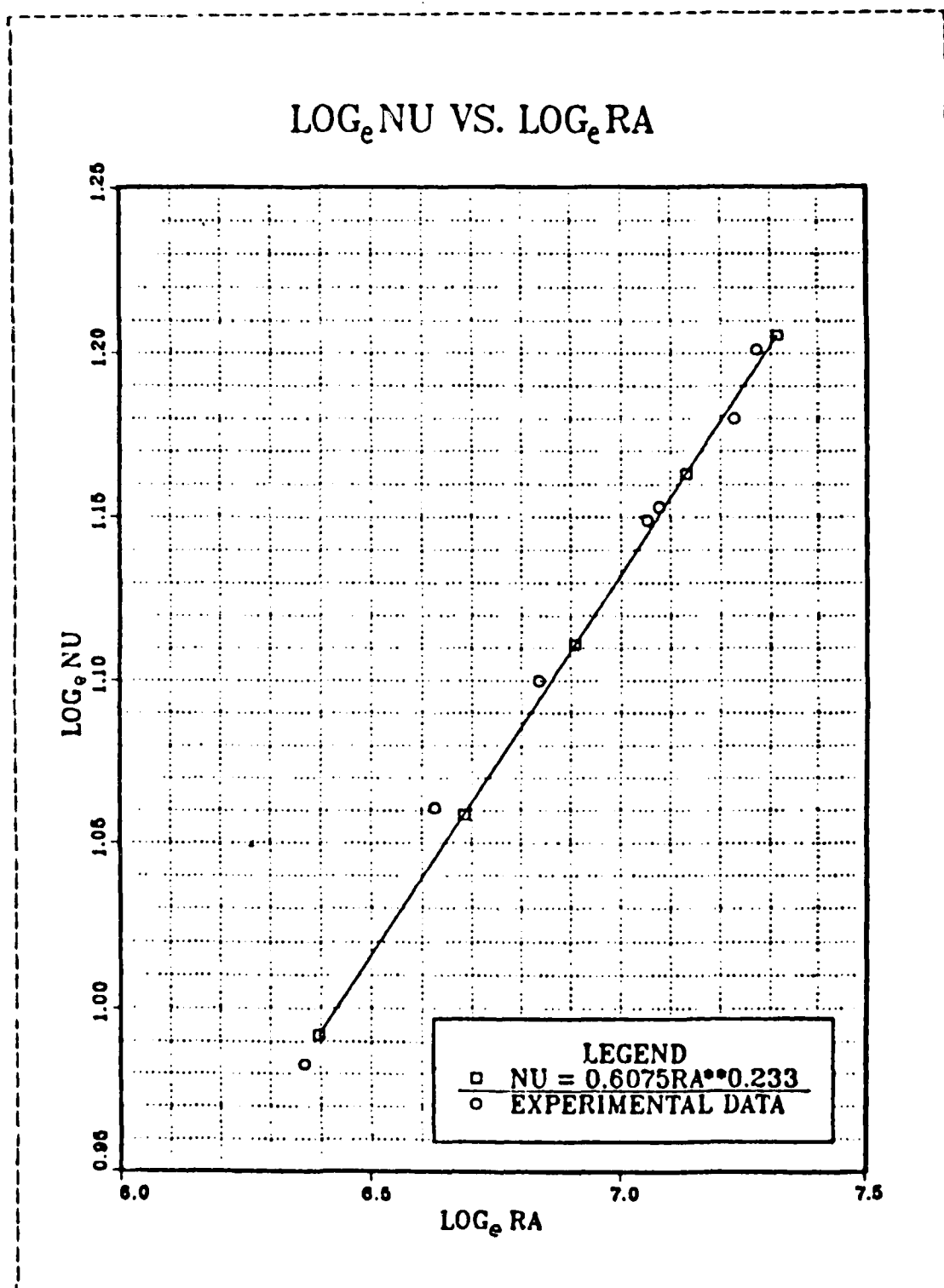
Figure B.3 \text{log}_e \text{Nu} vs. \text{log}_e \text{Ra} (20 degrees roll).
