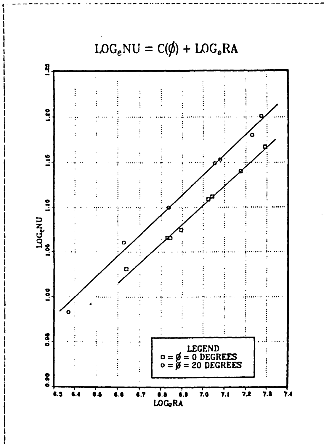
Figure B.6 Comparison of 0^\circ and 20^\circ Results.
