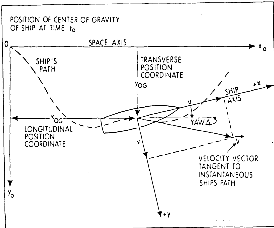
Figure 6.8 Orientation of Space Axes and Moving Axes.
