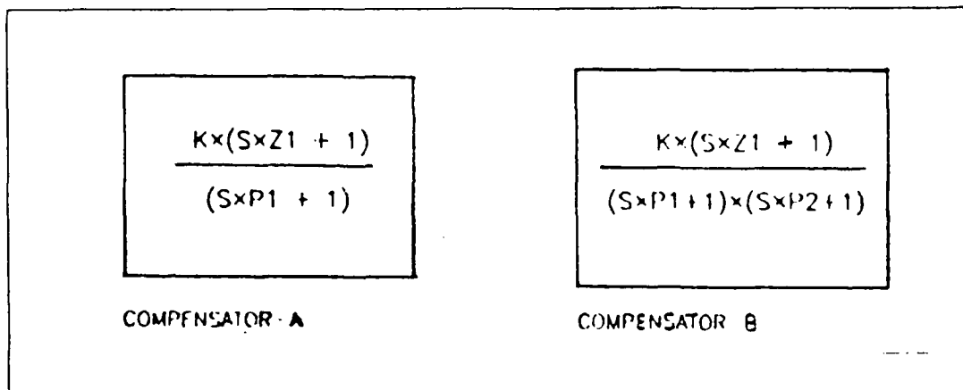
Figure 6.1 Various Structure Controllers.
