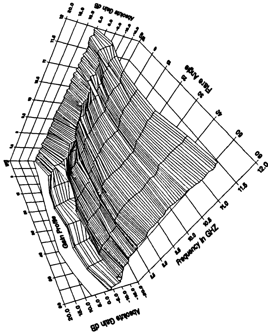
Figure 5.4 Gain Analysis Plot for Large B Antenna.
