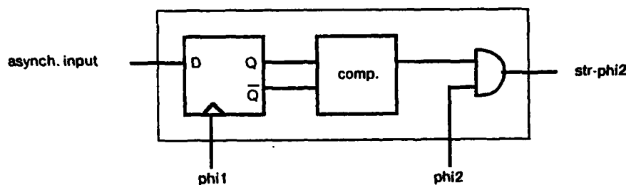
Figure 13. A synchronizer with metastability detection
