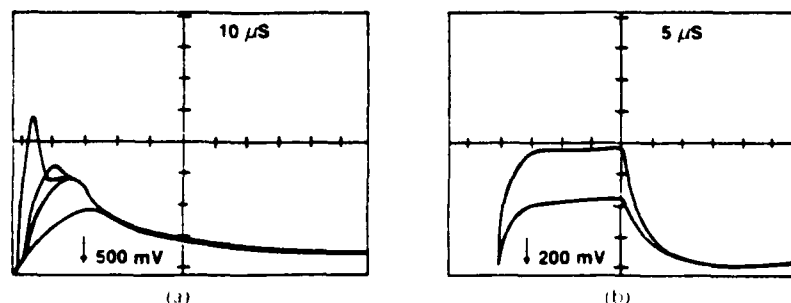
Fig. 26. Current decay in gas mixtures without (a) and with (b) attachments [93]. (a) Measured switch current in atmospheric pressure argon (10 \mu\text{s}/\text{div} horizontal, 5 A/div vertical) with electron beam current 20, 40, 80, 100 mA. (b) Measured switch current in atmospheric pressure argon with 0.02 Torr of \text{SF}_6 added (5 \mu\text{s}/\text{div} horizontal, 2 A/div vertical) with electron beam current 20, 50 mA [93].
