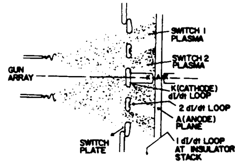
Fig. 32. Schematic of the plasma erosion switch (apparatus used in the Proto I experiment) [110].
