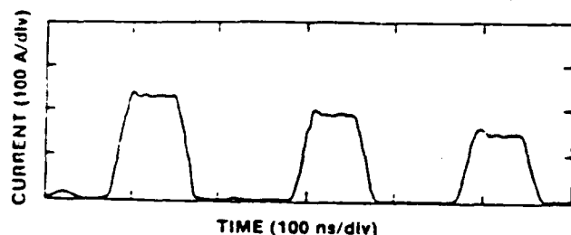
FIG. 3. e-beam current pulses measured at the cathode.
