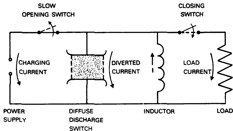
FIGURE 4. Schematic circuit for an e-beam sustained discharge switch in an inductive energy storage system.
