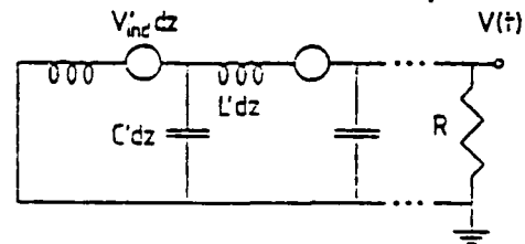
Fig. 1 Equivalent Circuit
