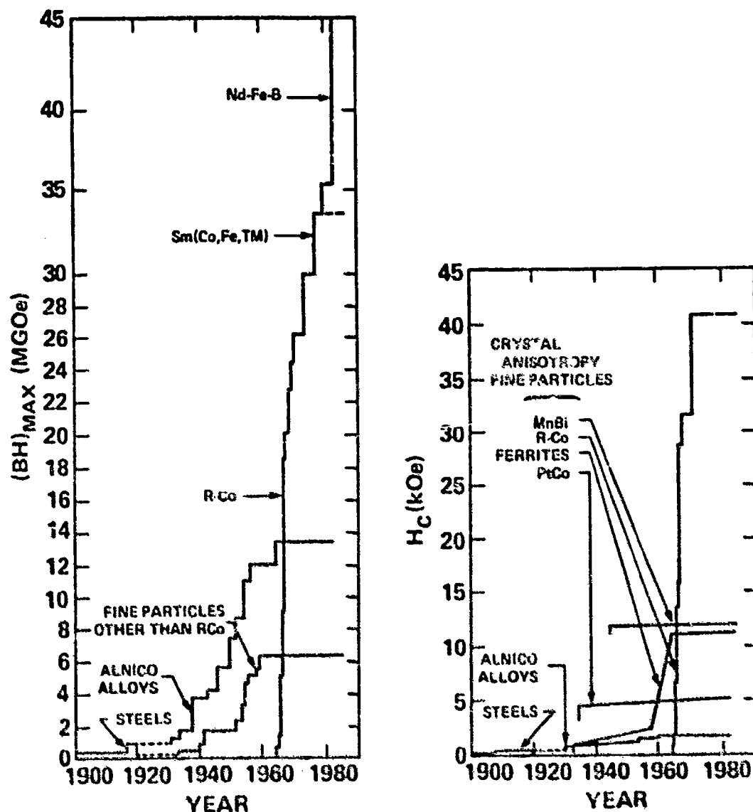
Figure 2 Energy product and coercivity of permanent magnets.
