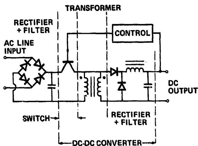
FIGURE 3 Simplified schematic diagram of typical off-line-switcher type power supply.
