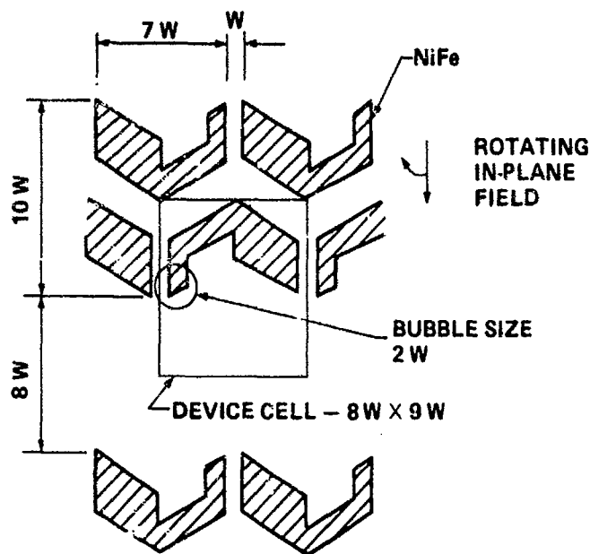
Figure 6 Bubble propagation structures showing device cell dimensions.
