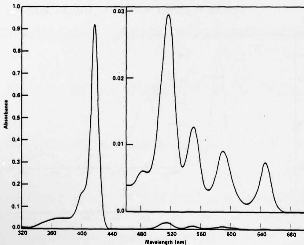
FIGURE 24: VISIBLE SPECTRUM OF MESO-TETRAPHENYL PORPHINE, TPP
