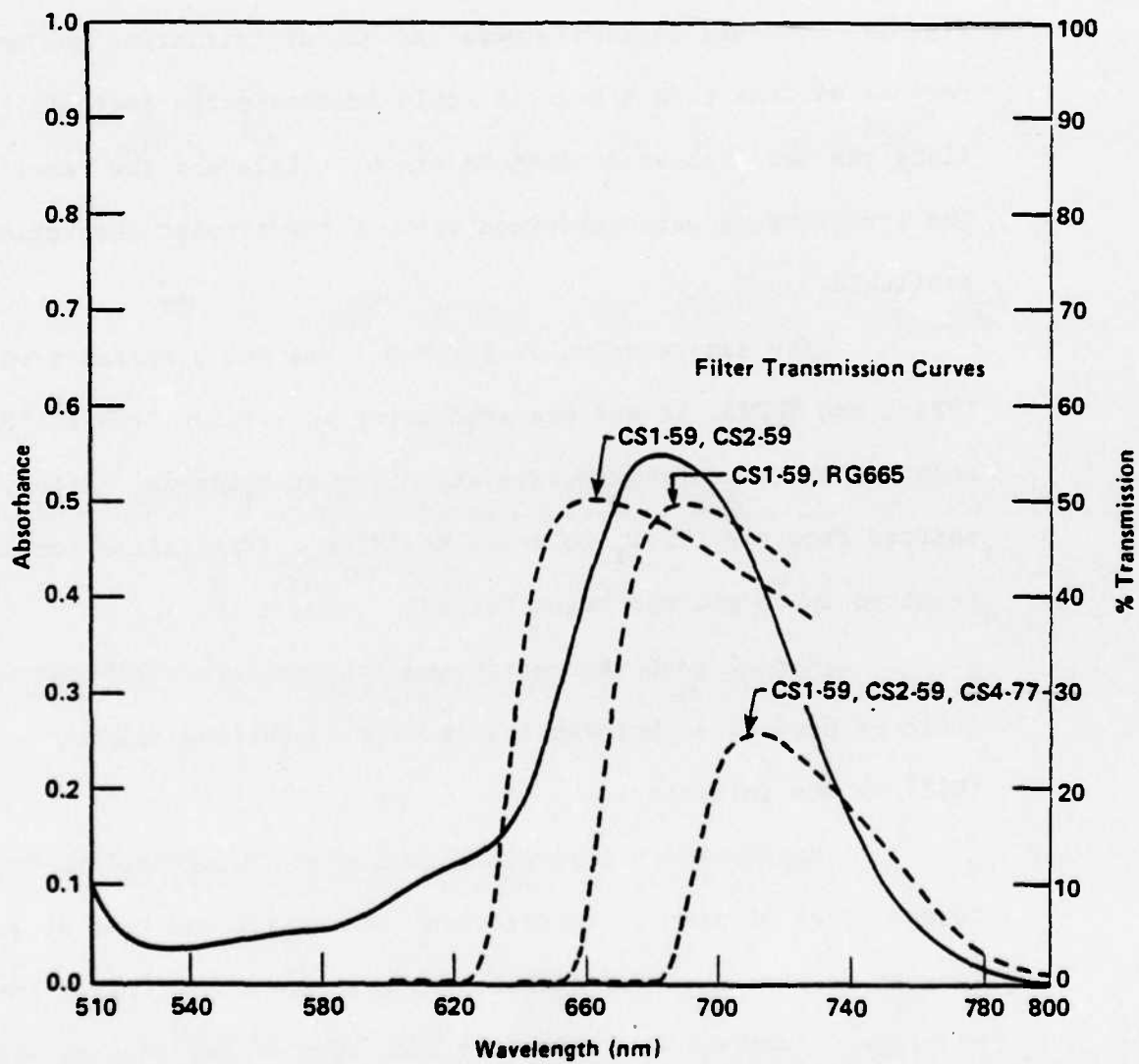
FIGURE 34: TPPBr X SPECTRUM + IRRADIATION FILTER CURVES
