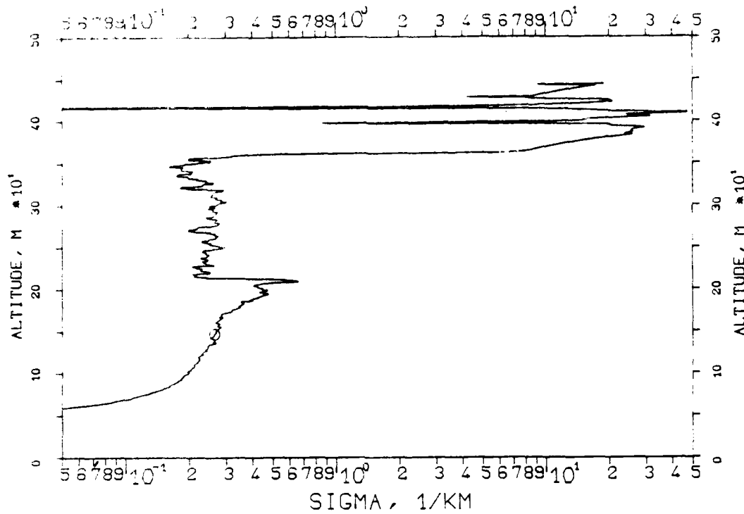
FIG. 7.247 KLETT-PROFILE, 0530NM, EL. 30DG00MN 341203, 12:47-12:47, CET RM=1.095KM, SM=20.0000/KM, K=1.000
