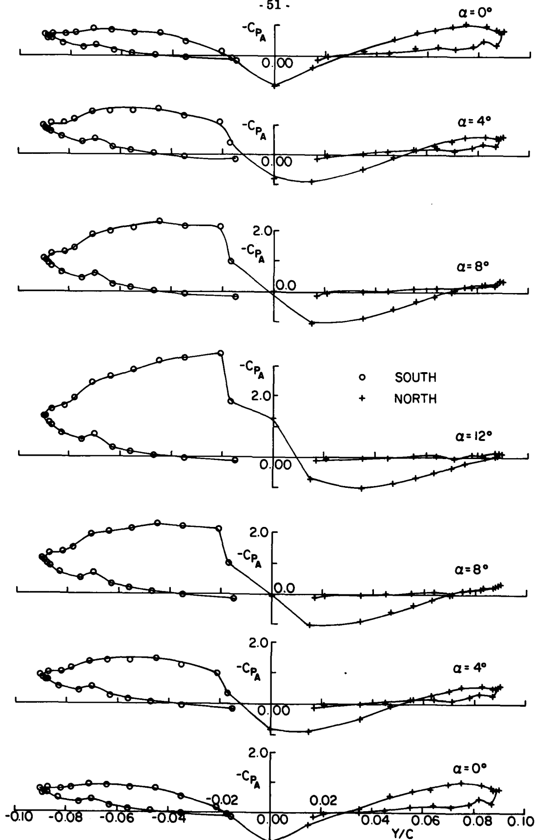
FIG. 18a: WING THICKNESSWISE PRESSURES DURING POSITIVE HALF-CYCLE, \alpha_m = \pm 12^\circ, \frac{R\Omega}{V} = 5, f = 0.55 \text{ Hz}
