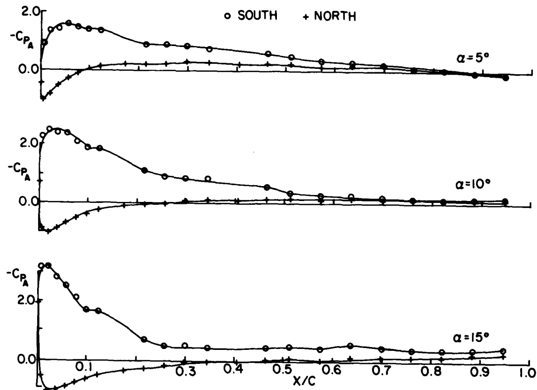
FIG. 13a: WING CHORDWISE PRESSURES DURING POSITIVE HALF-CYCLE, \alpha_m = \pm 20^\circ , \frac{R\Omega}{V} = 3 , f = 0.55 hz
