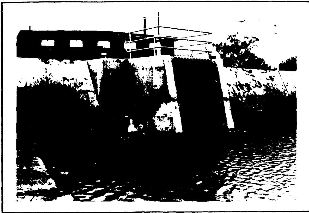
5. INLET DETAILS FOR THE 4-FOOT WIDE BY 6-FOOT HIGH IMPOUNDMENT REGULATING GATE APPROXIMATELY 110 FEET LEFT OF THE LEFT SIDE SPILLWAY ABUTMENT. (11/12/79)
