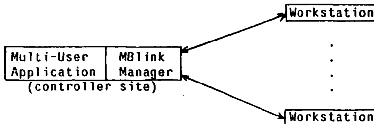
Figure 6-2: Architecture of Shared Bitmap System
