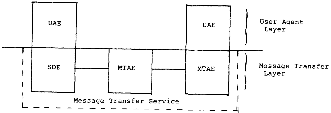
Figure 3-2: Alternate model showing layers, entities, and their relationships.
