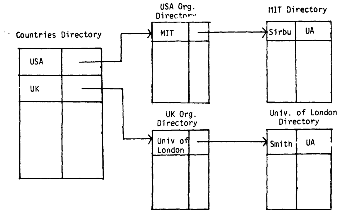
Figure 4-2: Multi-Component Names as Path Names
