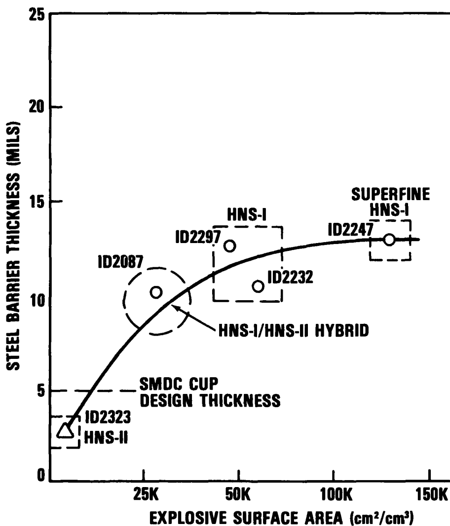
FIGURE 20. HEXANITROSTILBENE—FRAGMENT INITIATION SENSITIVITY AT A 50% FIRE RESPONSE WITH STEEL BARRIER THICKNESS VERSUS EXPLOSIVE SURFACE AREA AT THE 0", 100 AIR GAP (SIDE-TO-END CONFIGURATION)
