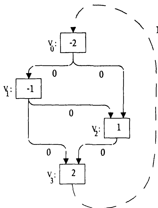
Figure 5-3: Example Min-Cost Flow Problem
