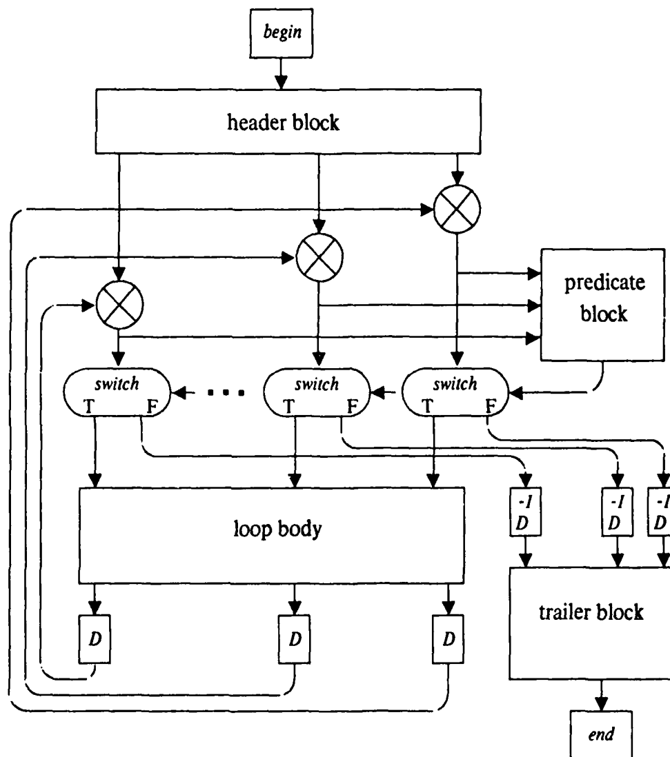
Figure 2-6: Loop Code-block Schema
