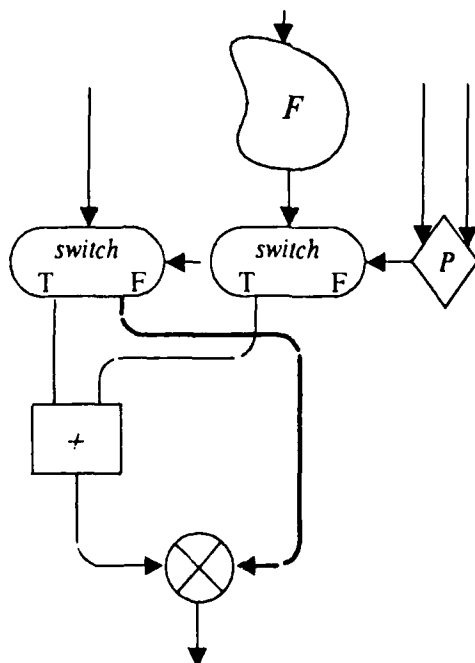
Figure 4-1: Typical Termination Problem
