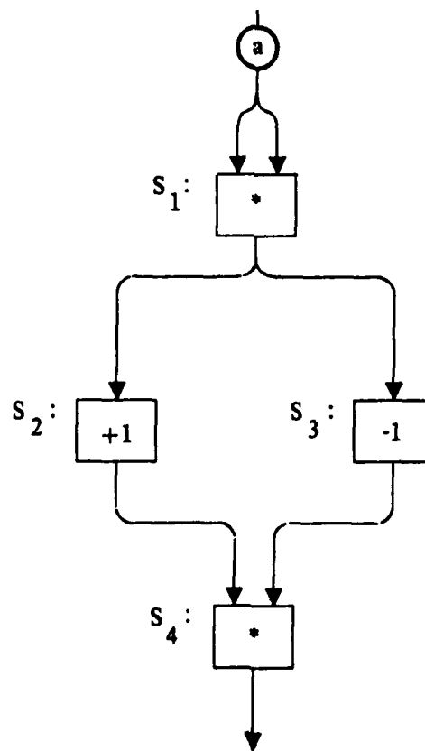
Figure 2-1: A Simple Dataflow Graph
