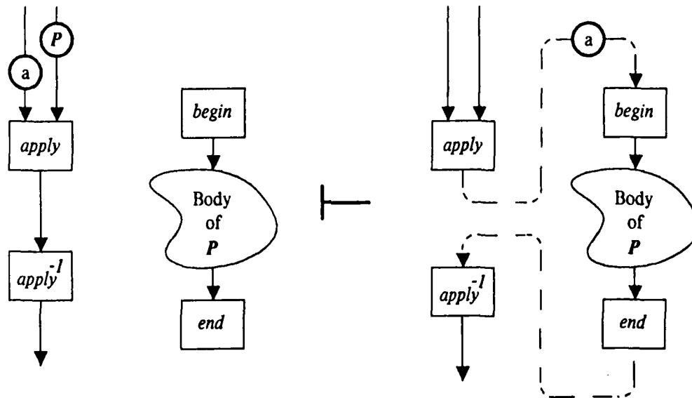
Figure 2-4: Code-block Invocation
