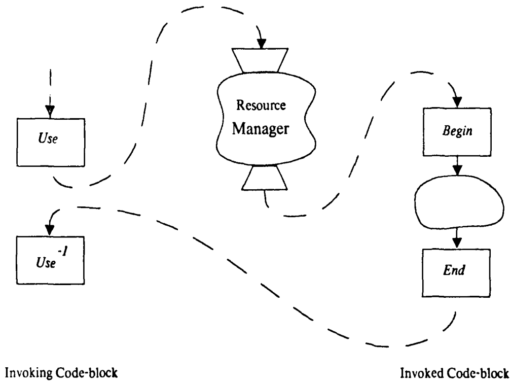
Figure 3-4: Use Schema
