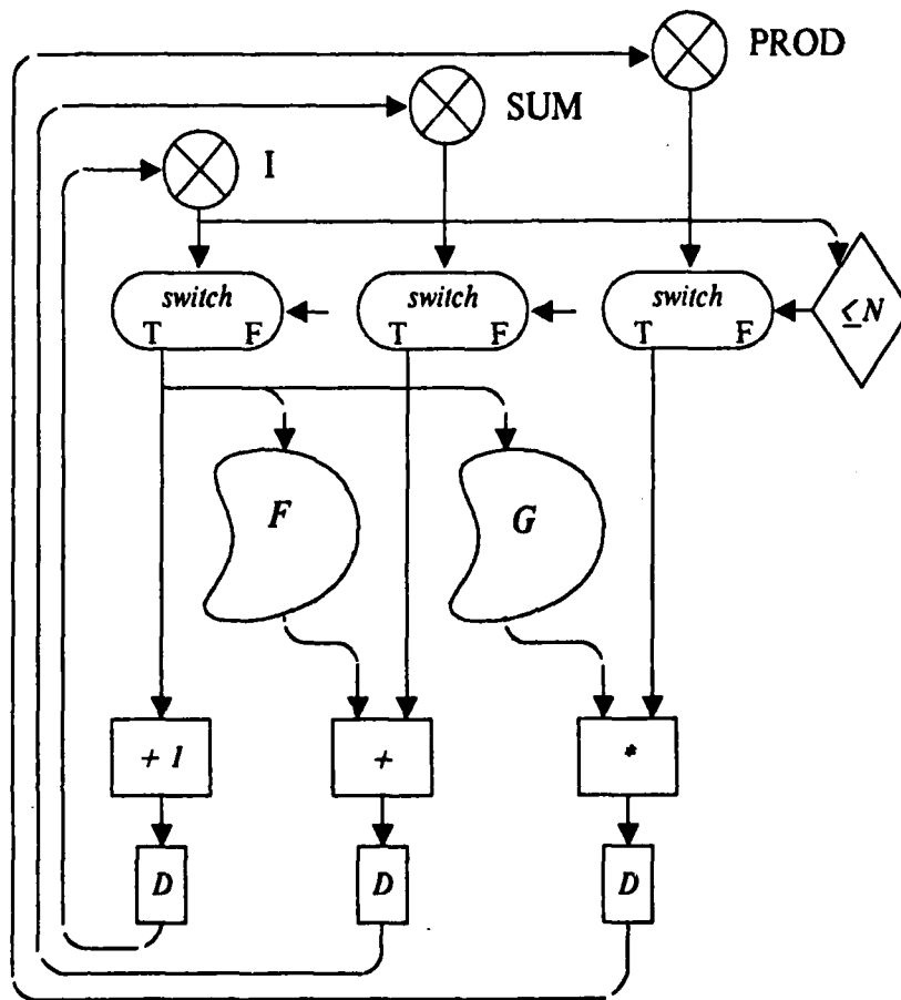
Figure 7-4: Unbounded Loop
