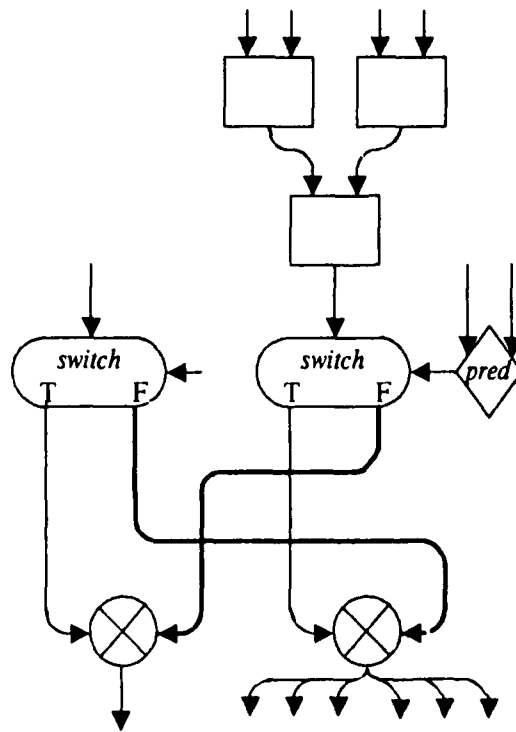
Figure 6-1: Sub-Block Replacement Counter Example
