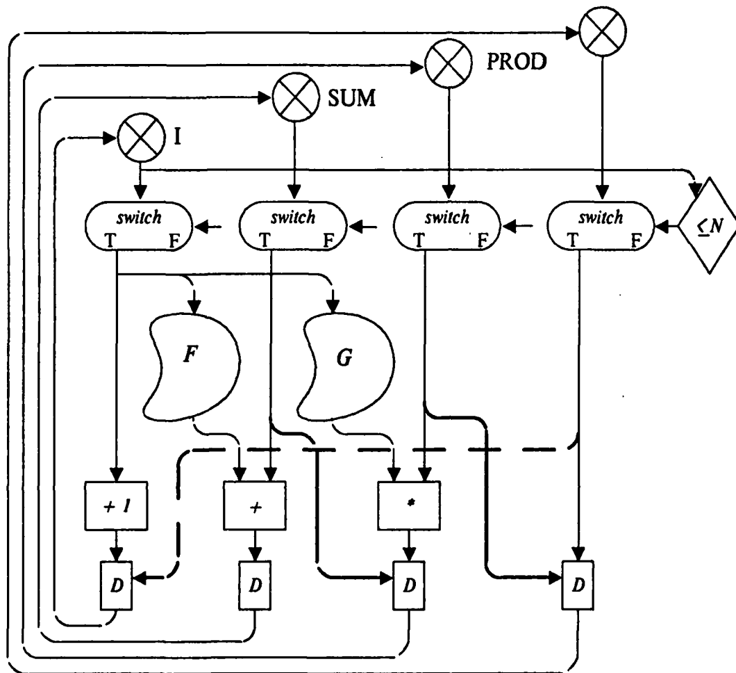
Figure 7-8: Auxiliary Loop Variables
