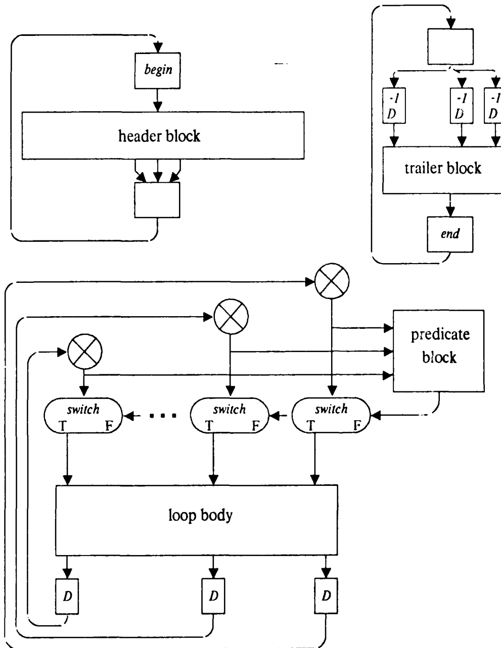
Figure 7-1: Loop Broken Down for Analysis
