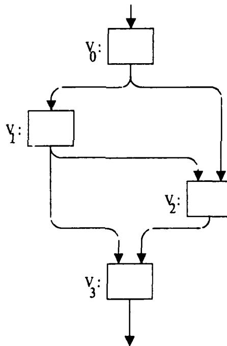
Figure 5-1: Basic Acyclic Block
