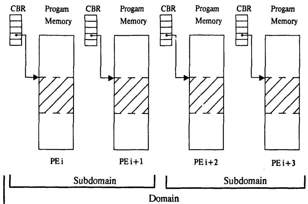
Figure 3-3: Allocation of Program Memory
