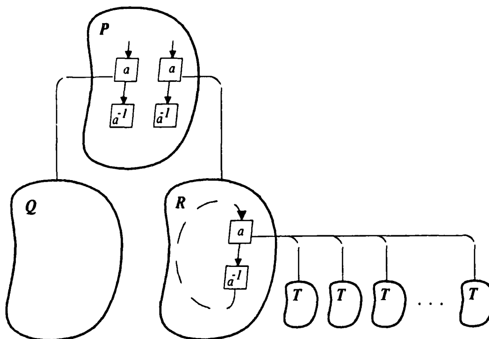
Figure 2-8: Invocation Tree with Loop Code-blocks
