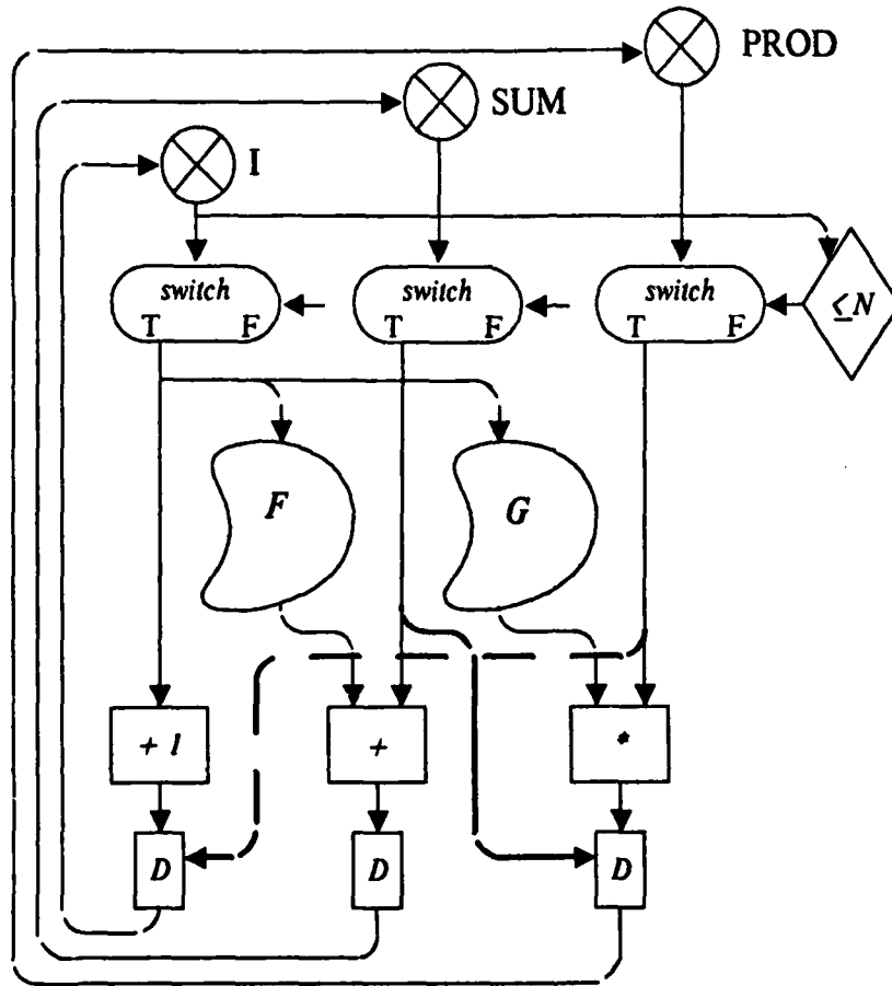
Figure 7-6: Transformed (Bounded) Loop
