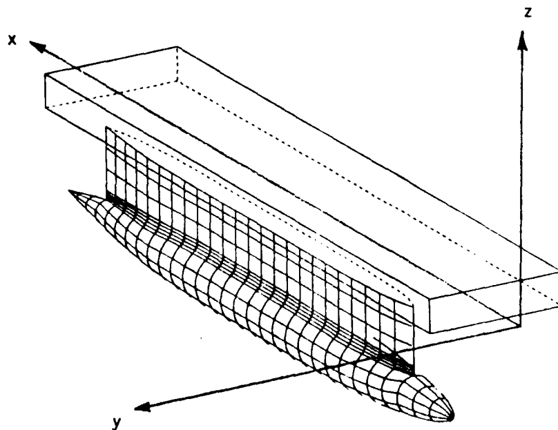
Figure A-1. Global coordinate system.
