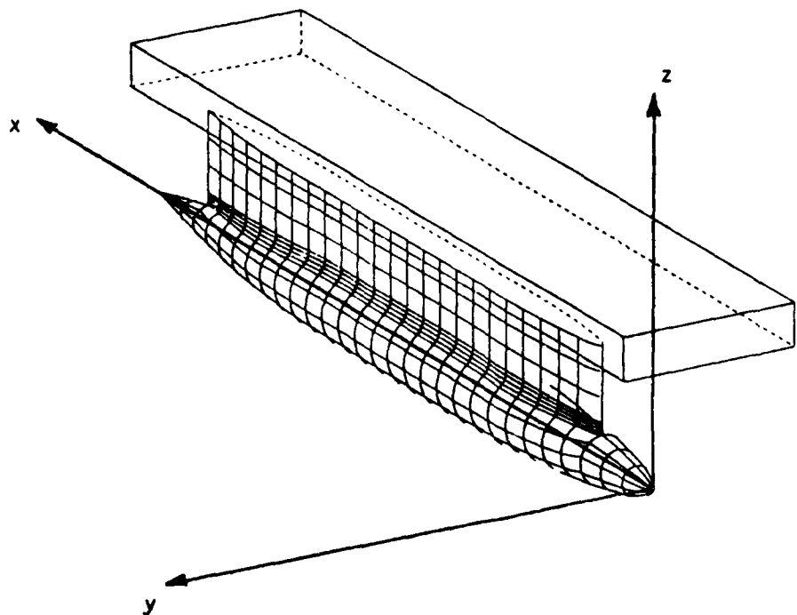
Figure A-3. Lower hull local coordinate system.
