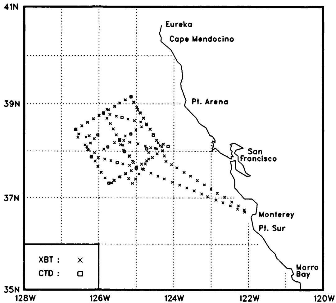
Figure 14: XBT and CTD locations for OPTOMAl1, Leg AII.
