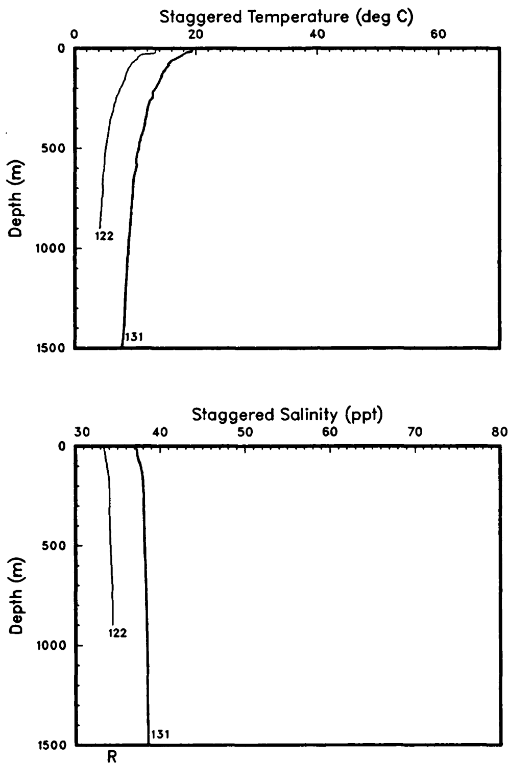
Figure 48: CTD casts deeper than 800m. (OPTOM11, Leg DII).
