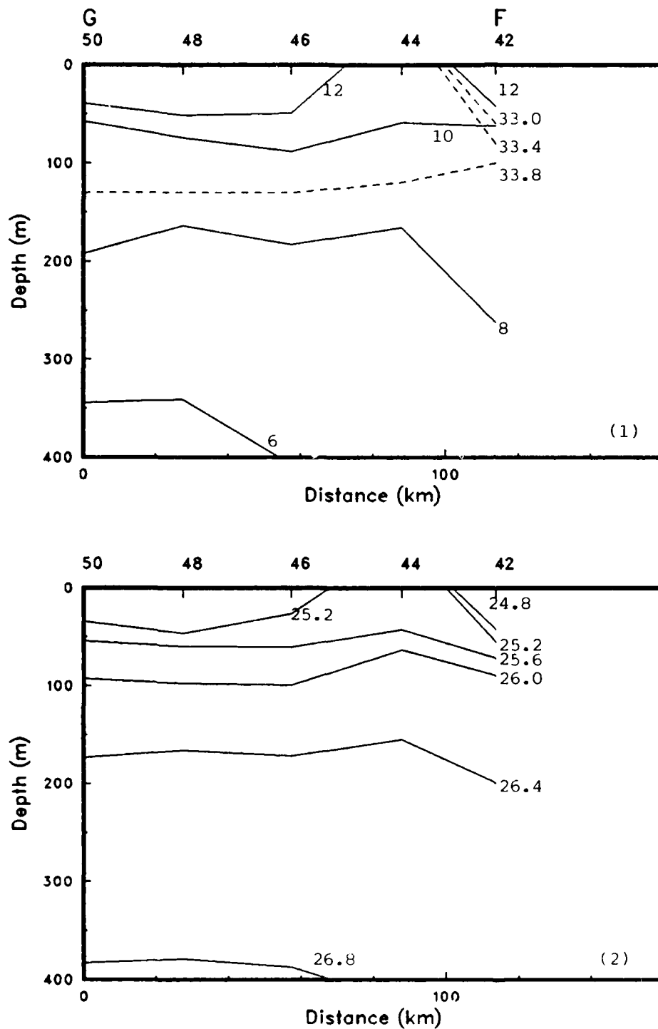
Figure 63(a): Isopleths of (1) temperature and salinity and (2) sigma-t from the CTD's. (OPTOMA11, Leg DIII).
