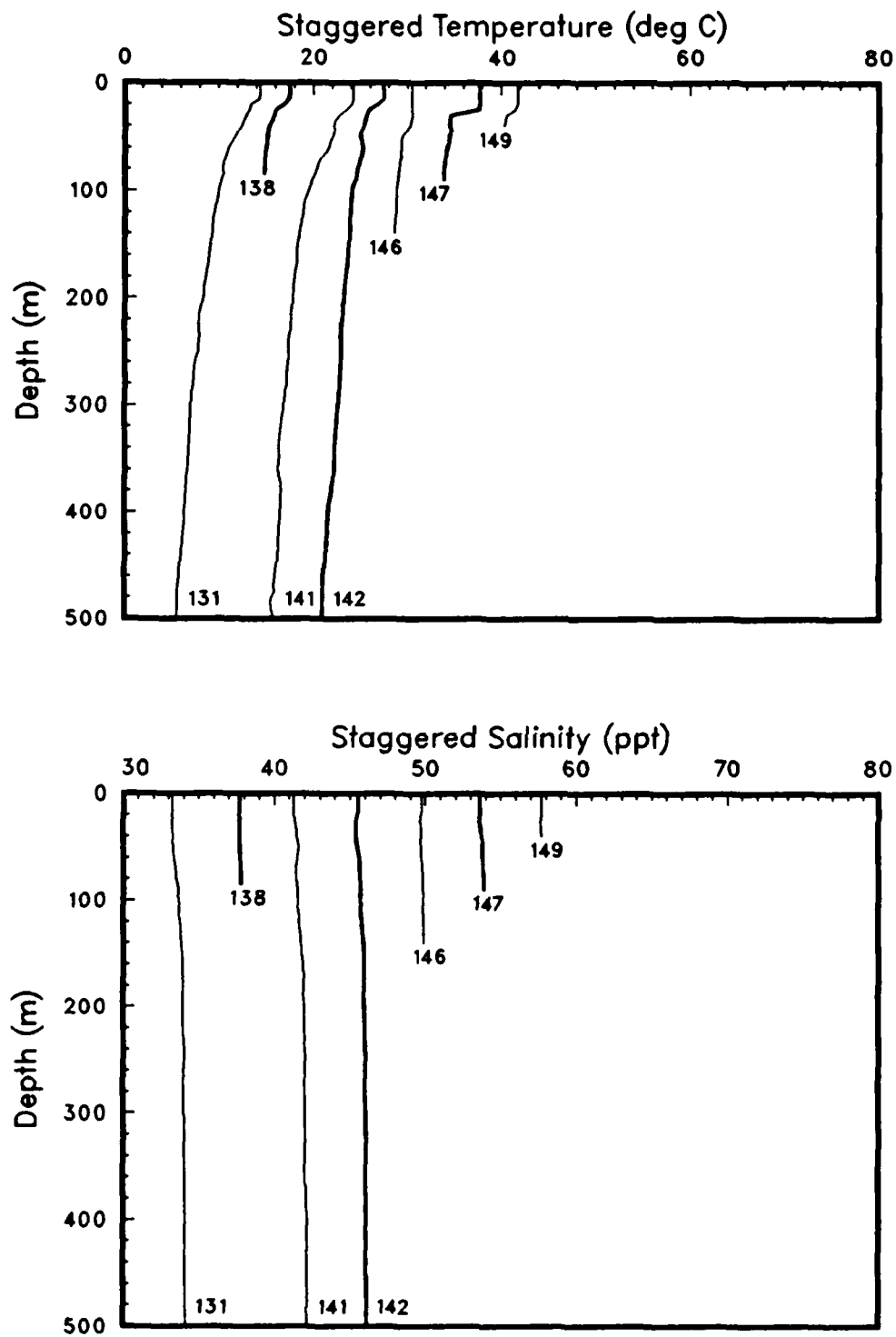
Figure 49: Nearshore CTD casts plotted to 500m or less. (OPTOMA11, Leg DII).
