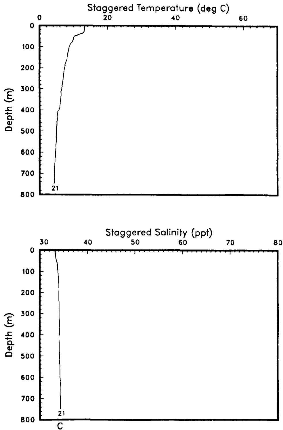
Figure 28: CTD temperature and salinity profiles. (OPTOMAl1, Leg AIII).
