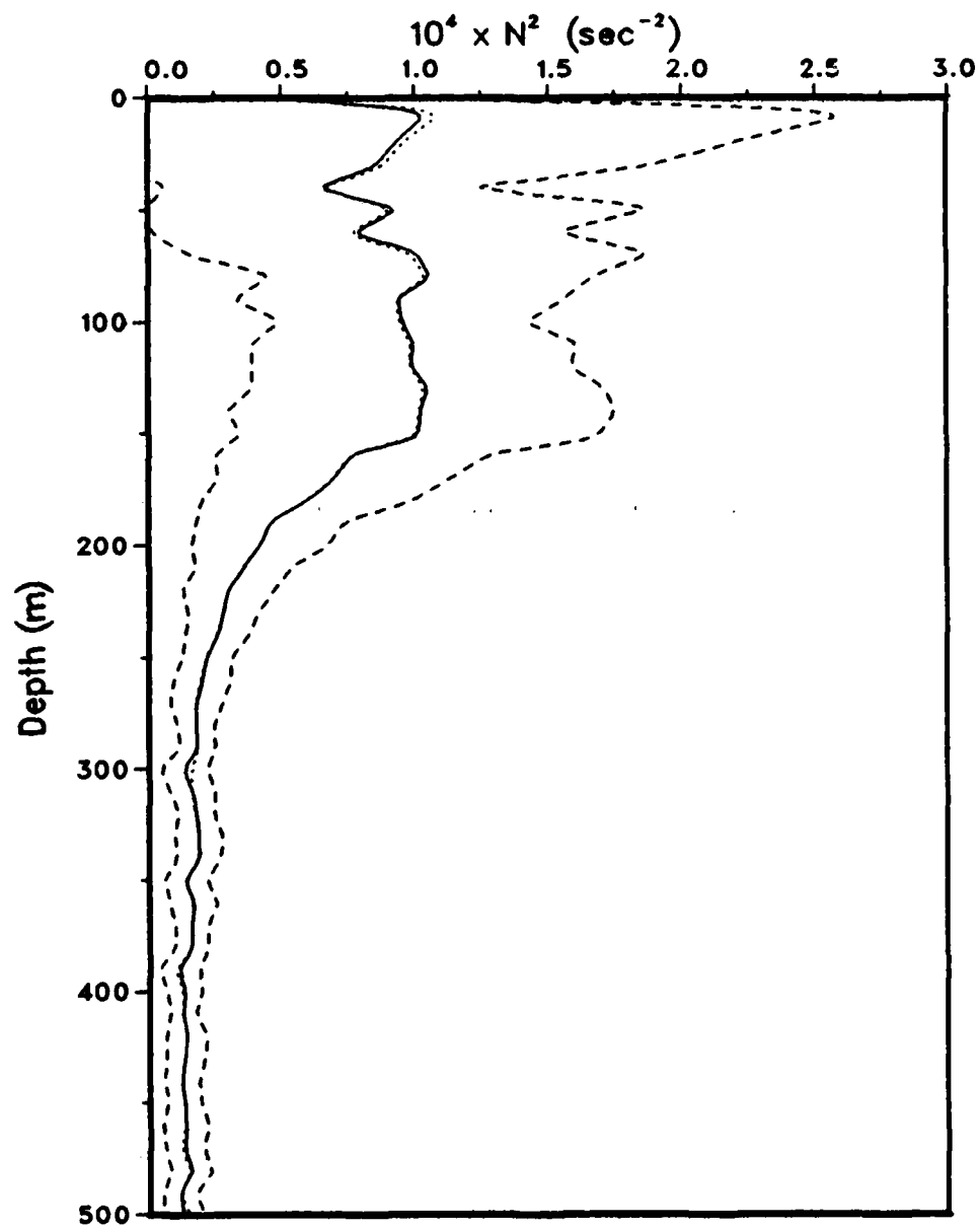
Figure 42: Mean N^2 profile (—), with + and - the standard deviation (----). The N^2 profile from \overline{T(z)} and \overline{S(z)} is also shown (.....). (OPTOMAll, Leg DI).
