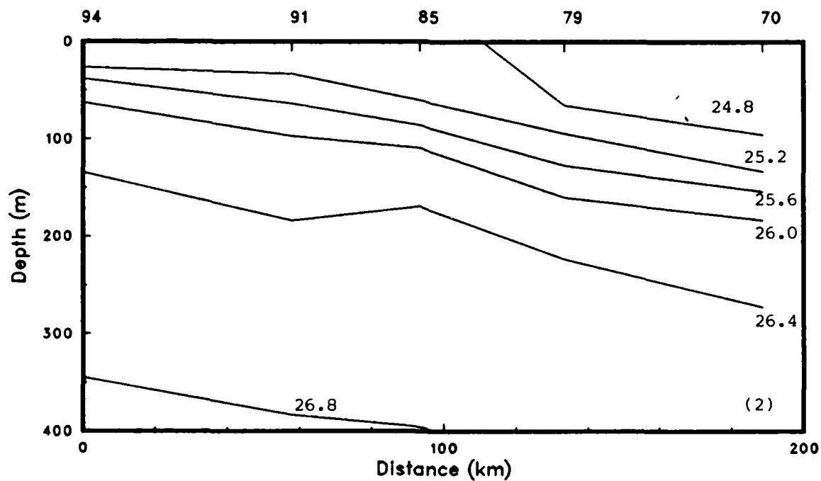
Figure 51(a): Isopleths of (1) temperature and salinity and (2) sigma-t from the CTD's. (OPTOMA11, Leg DII).
