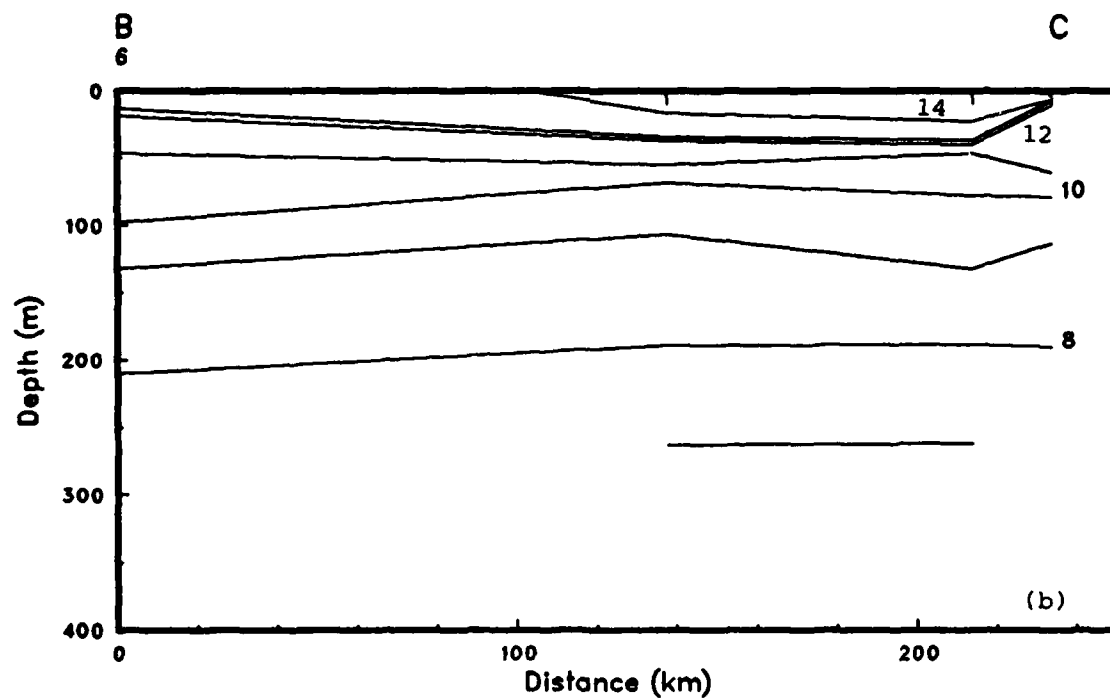
Figure 72(a), (b): Along-track isotherms. Tick marks along the upper horizontal axis show station positions. Some station numbers are given. Dashed lines are used if the cast was too shallow. (OPTOMA11, Leg P).
