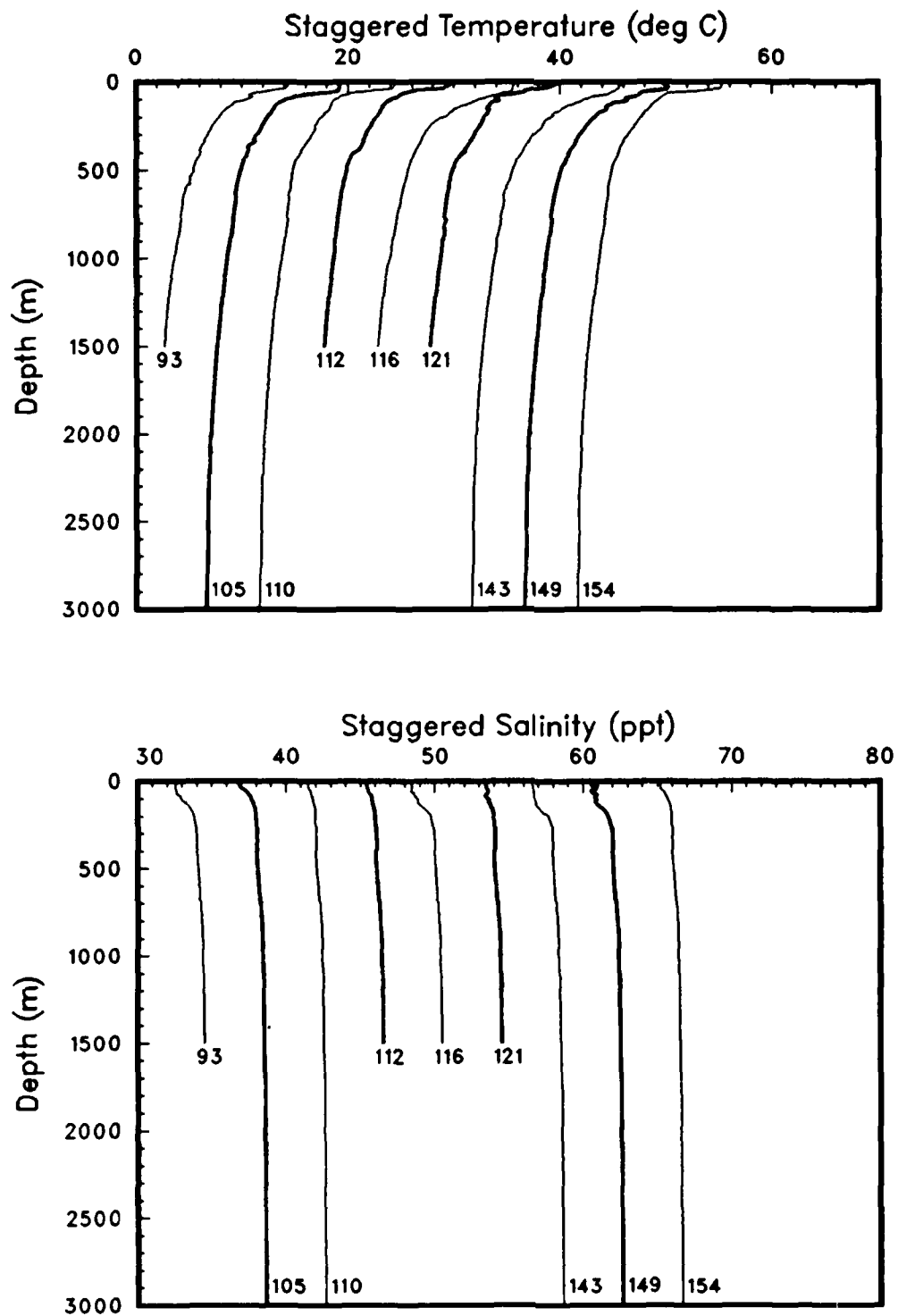
Figure 61: CTD casts deeper than 800m. (OPTOMA11, Leg DIII).
