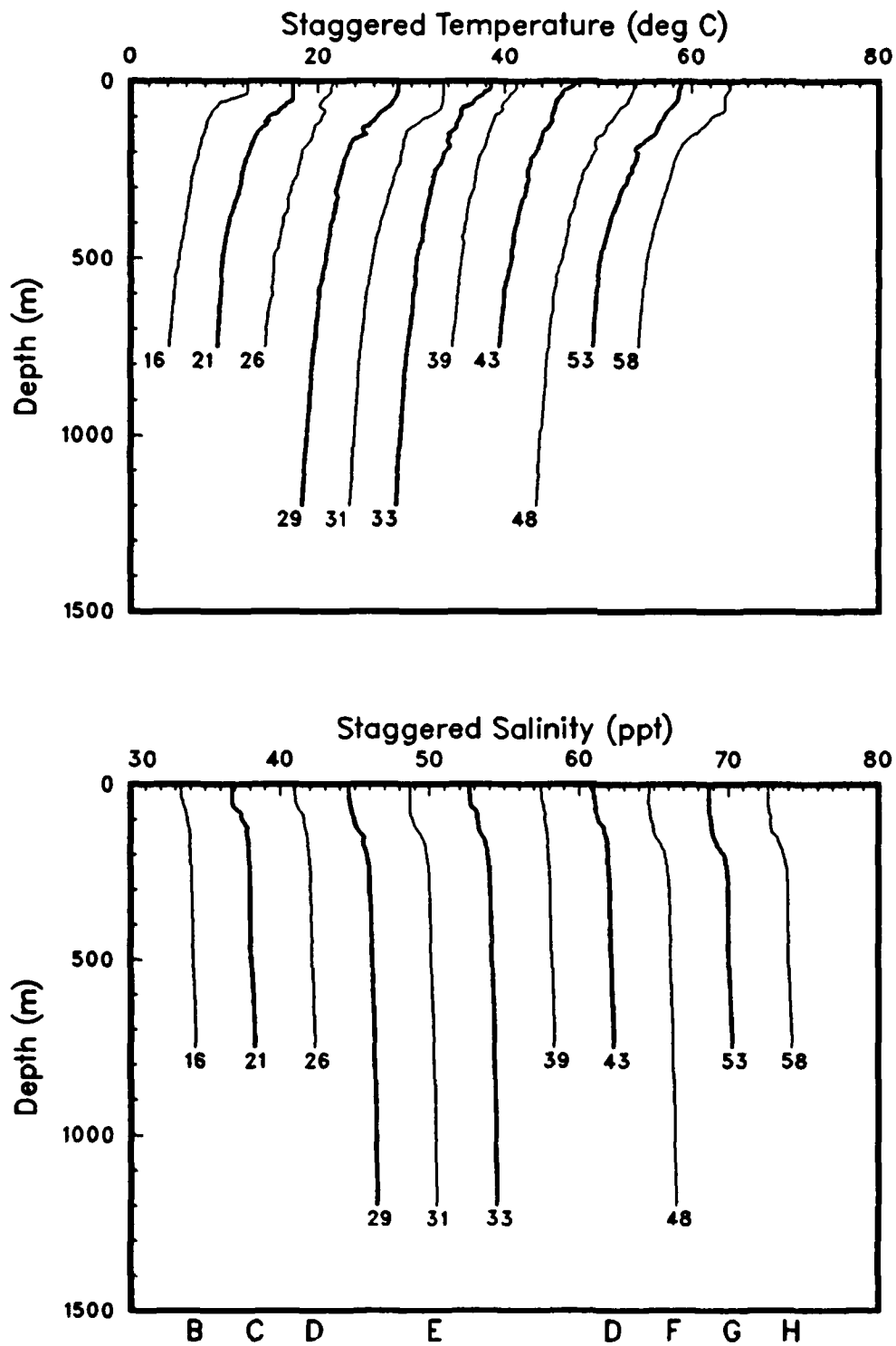
Figure 17(a): CTD temperature profiles, staggered by multiples of 5C, and salinity profiles, staggered by multiples of 4 ppt. (OPTOMAll, Leg AII).
