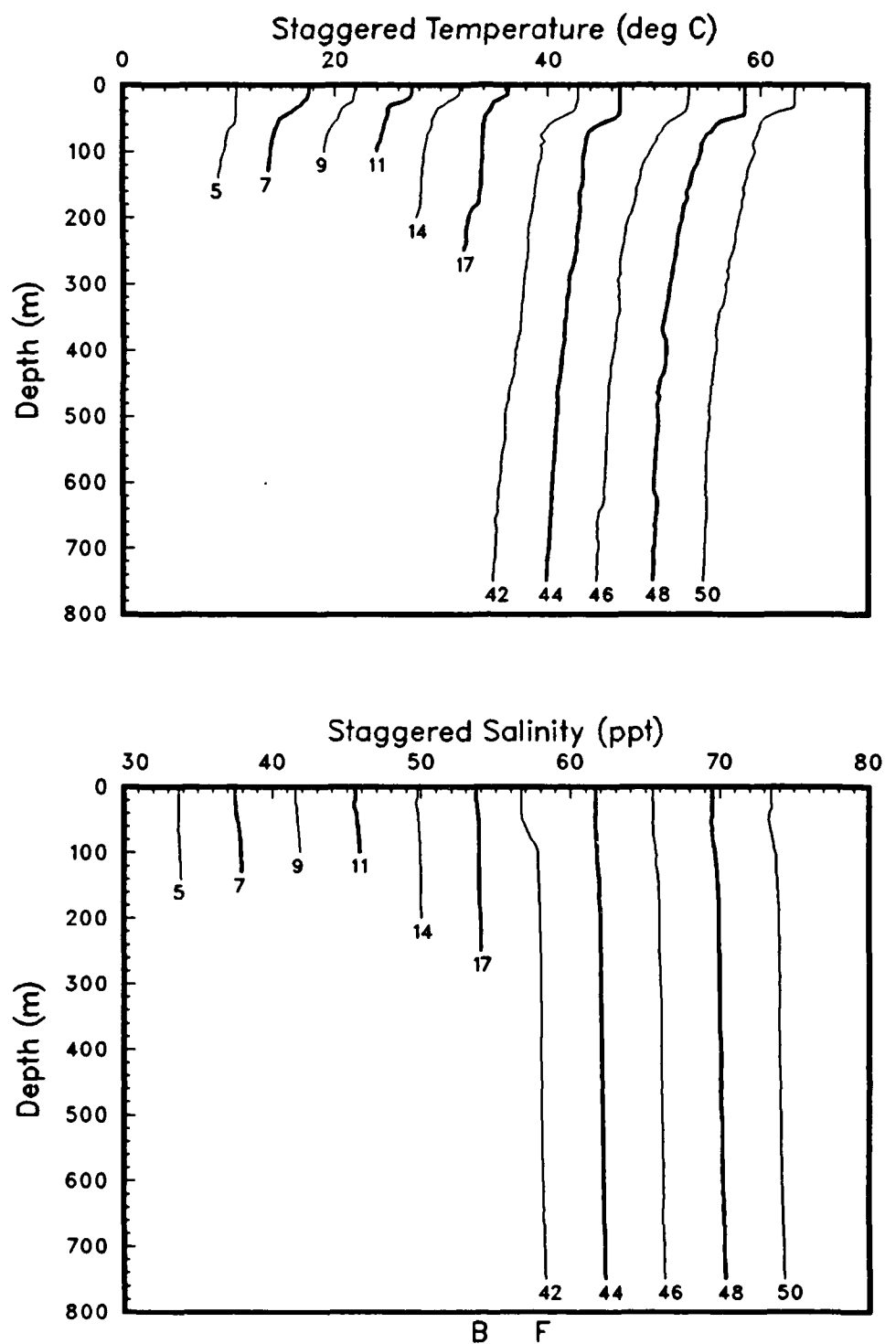
Figure 60(a): CTD temperature profiles, staggered by multiples of 5C, and salinity profiles, staggered by multiples of 4 ppt. (OPTOMAll, Leg DIII).
