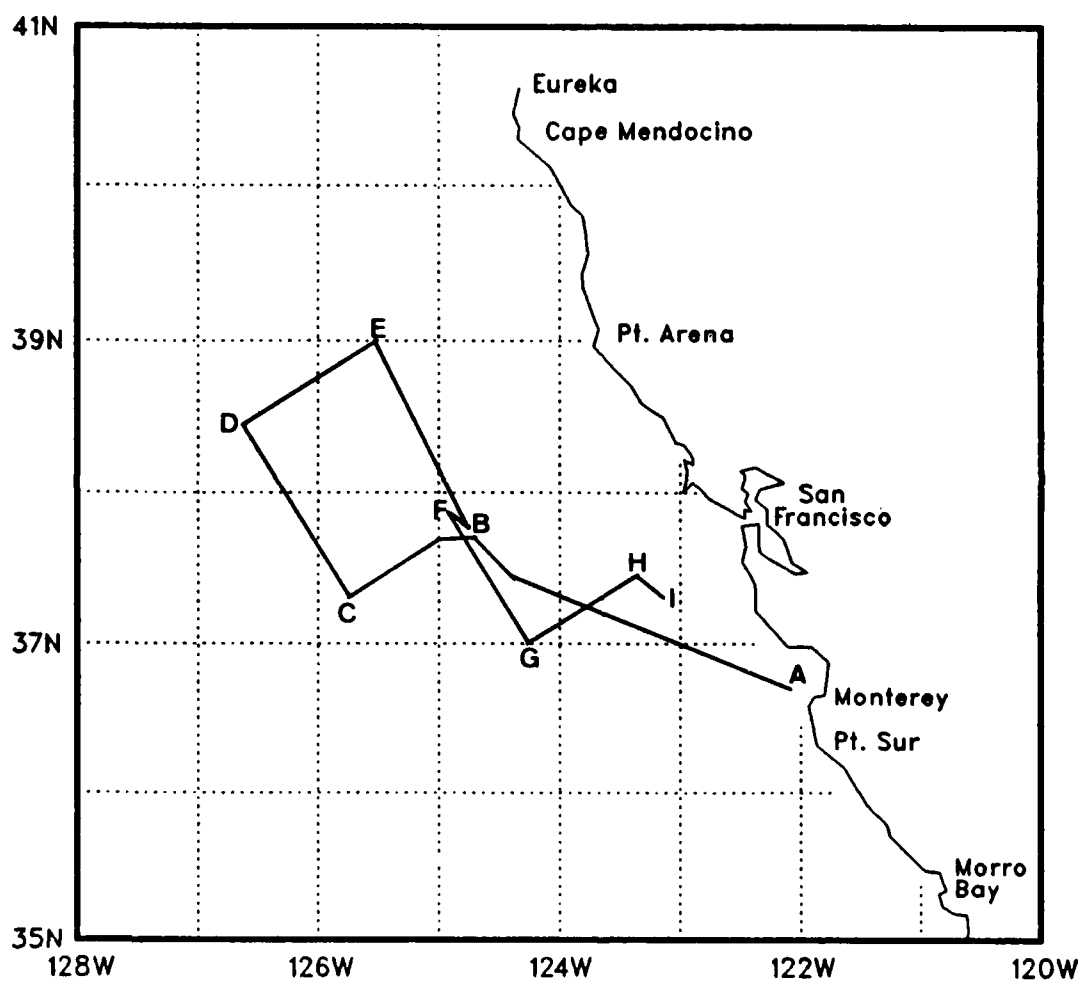
Figure 24: The cruise track for OPTOMAl1, Leg AIII.
