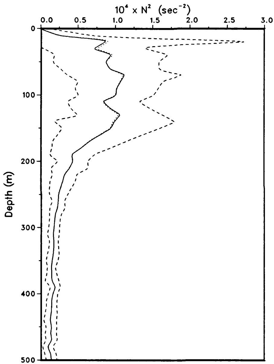
Figure 55: Mean N^2 profile (—), with + and - the standard deviation (----). The N^2 profile from \overline{T(z)} and \overline{S(z)} is also shown (.....). (OPTOMAl1, Leg DII).
