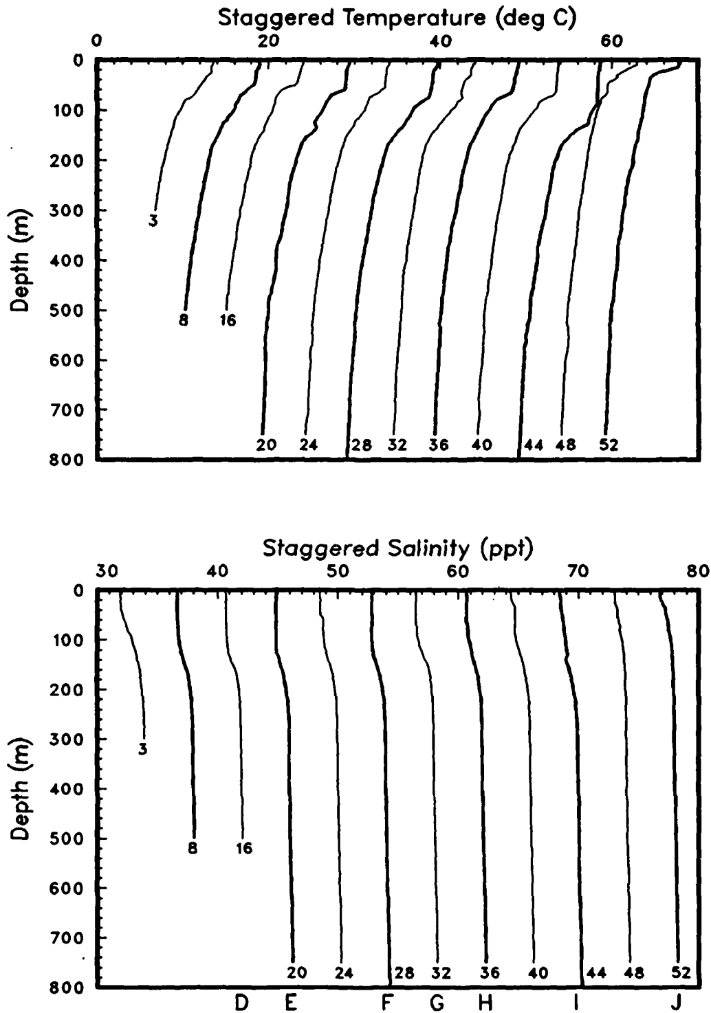
Figure 35(a): CTD temperature profiles, staggered by multiples of 5C, and salinity profiles, staggered by multiples of 4 ppt. (OPTOM11, Leg DI).
