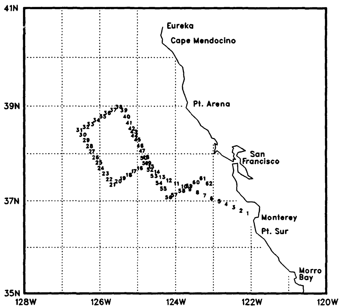
Figure 26: Station numbers for OPTOMAll, Leg AIII.
