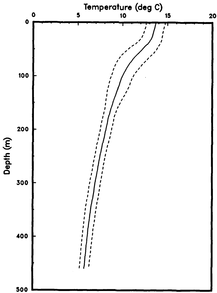
Figure 30: Mean temperature profile, with + and - the standard deviation. (OPTOMAl1, Leg AIII).
