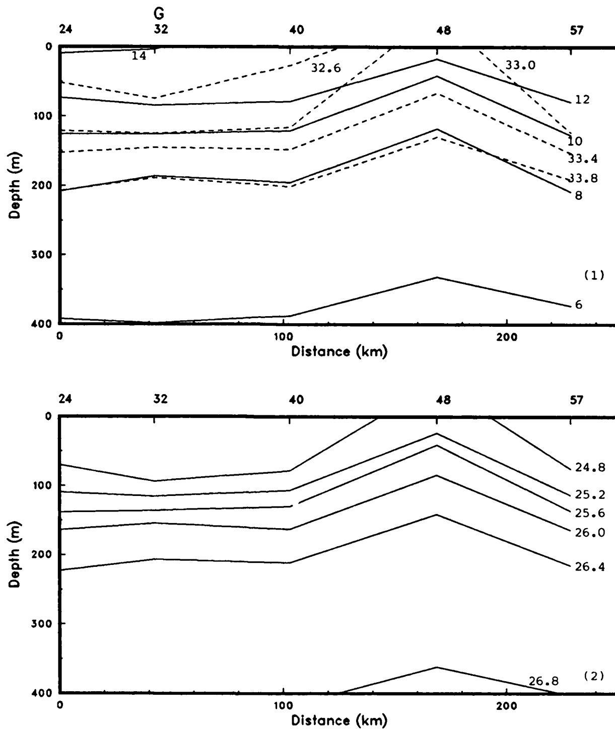
Figure 38(a): Isopleths of (1) temperature and salinity and (2) sigma-t from the CTD's. Dotted lines are used if the cast was too shallow. (OPTOMAll, Leg DI).
