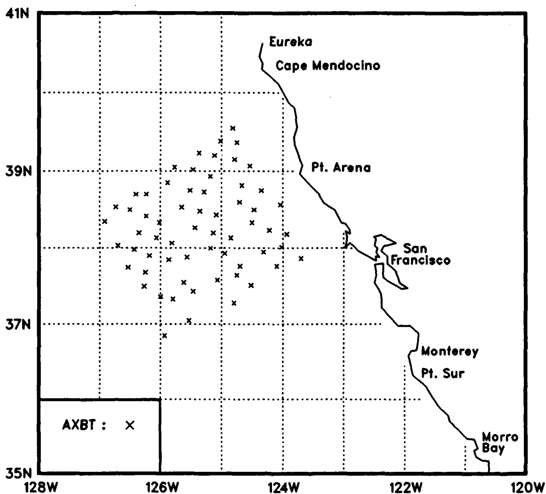
Figure 69: AXBT locations for OPTOMAl1, Leg P.
