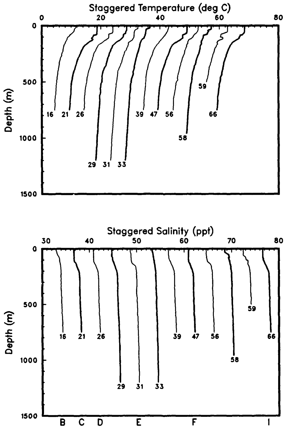
Figure 6(a): CTD temperature profiles, staggered by multiples of 5C, and salinity profiles, staggered by multiples of 4 ppt. (OPTOMAll, Leg A1).
