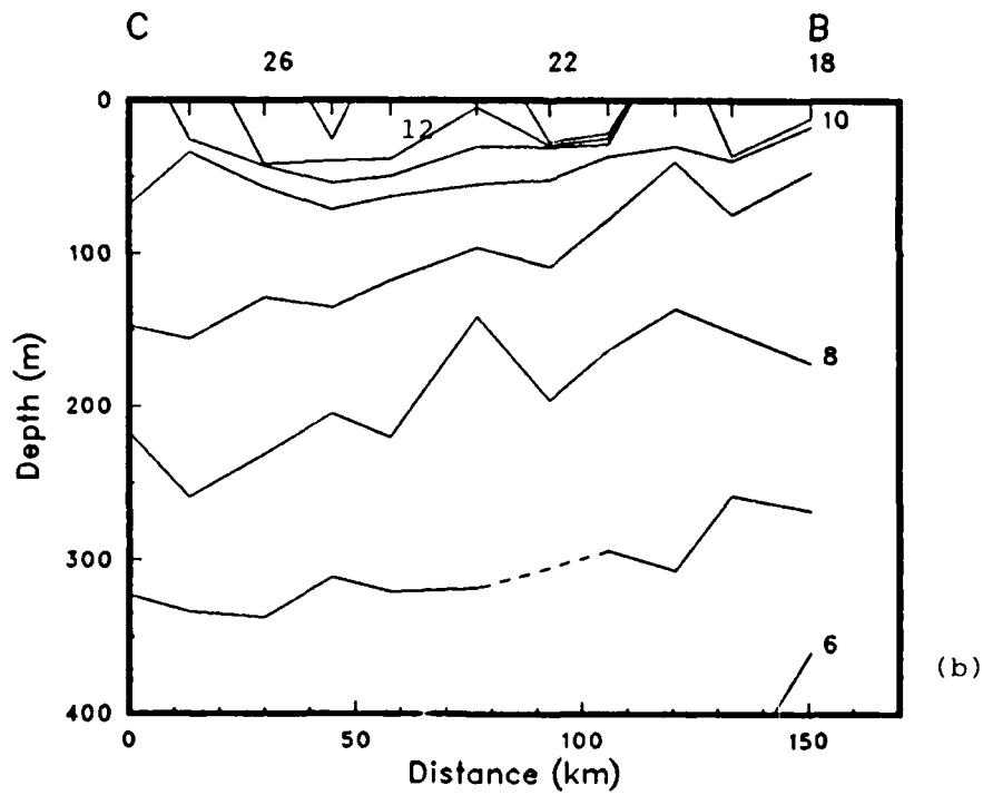
Figure 62(a), (b): Along-track isotherms. Tick marks along the upper horizontal axis show station positions. Some station numbers are given. Dashed lines are used if the cast was too shallow. (OPTOMA11, Leg DIII).
