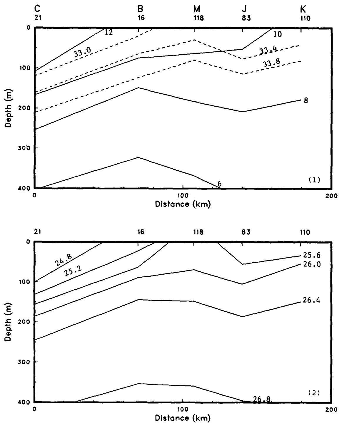
Figure 8(a): Isopleths of (1) temperature and salinity and (2) sigma-t from the CTD's. (OPTOMA11, Leg AI).
