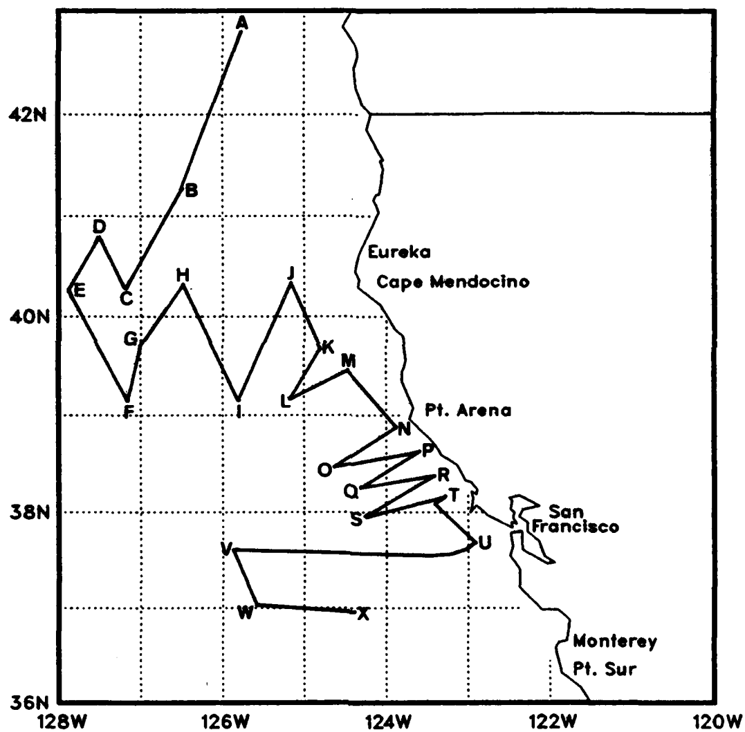
Figure 31: The cruise track for OPTOMAl1, Leg DI.
