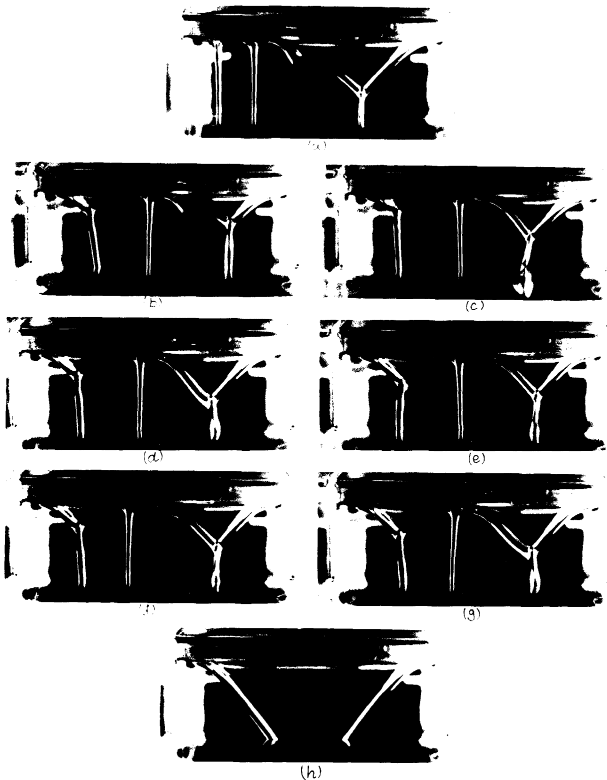
Fig. 21. The branch of (CT) flows. (a) The branch of flows lost stability to this unsteady (CT) flow at R = 1.4 , S = 12.7 , h = 3.43 mm, v = 0.792 St.; (b), (c): R = 1.55 , S = 12.0 , h = 3.43 mm, v = 0.792 St.; (d), (e): R = 1.75 , S = 11.8 , h = 3.55 mm, v = 0.786 St.; (f), (g): R = 1.86 , S = 11.2 , h = 3.65 mm, v = 0.793 St.; (h) the branch of flows lost stability to this steady (T) flow at R = 1.90 , S = 11.0 , h = 3.67 mm, v = 0.792 St.
