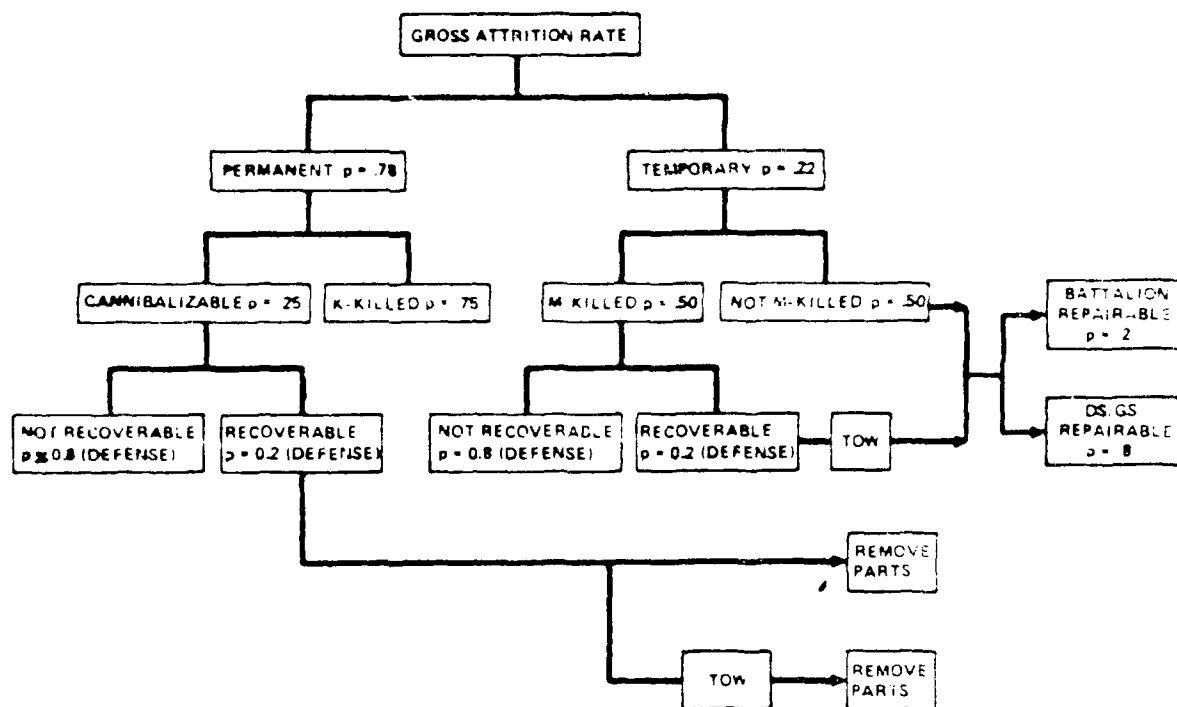
Fig. E.1—Attrition, battle damage, and recovery assumptions (M60A1 active defense)
