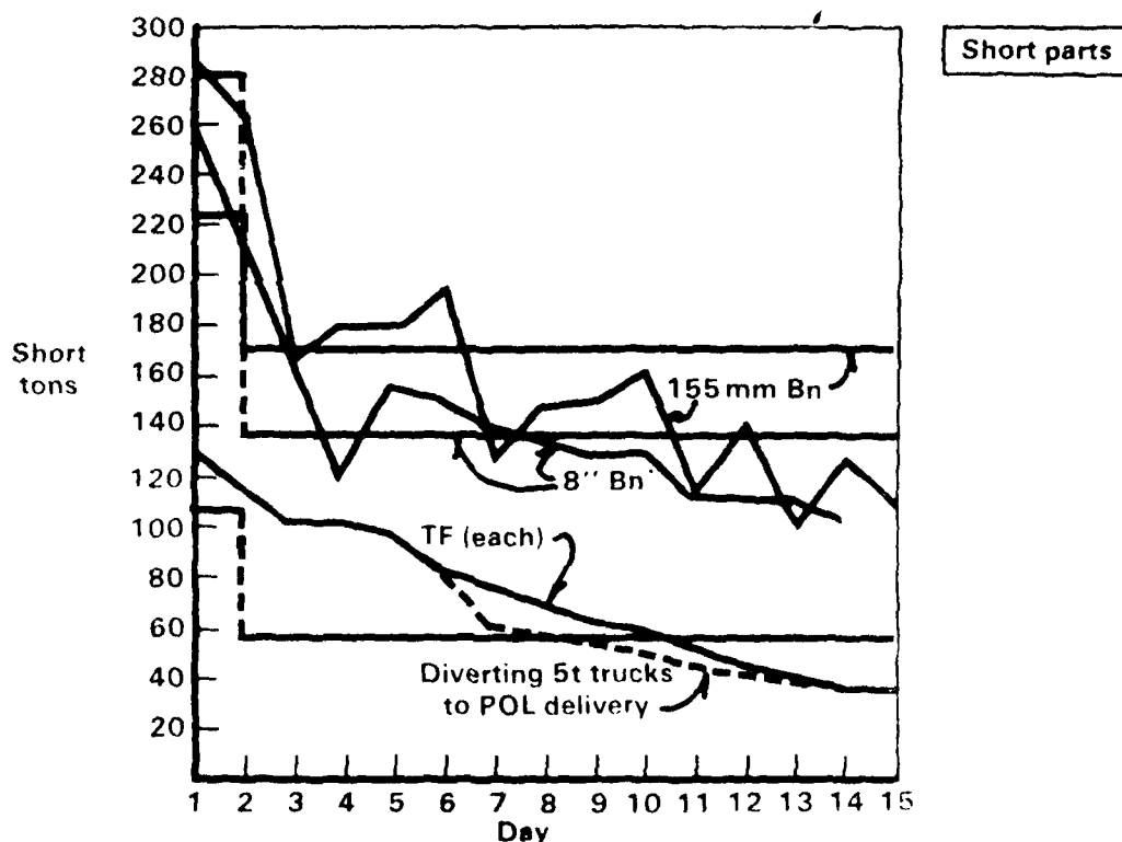
Fig. 3— Ammunition deliveries to consumption points (FULLTRUCK)
