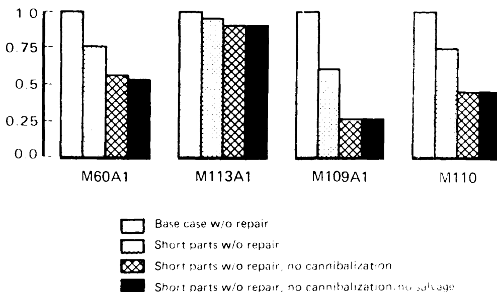
Fig. 20—Cannibalization and salvage: active defense SOC
