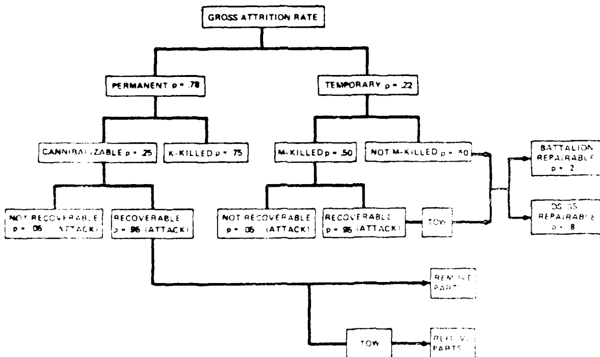
Fig. E.2—Attrition, battle damage, and recovery assumptions (M60A1 attack)
