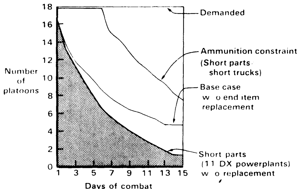
Fig. 9—Tank missions demanded/accomplished (active defense SOC)
