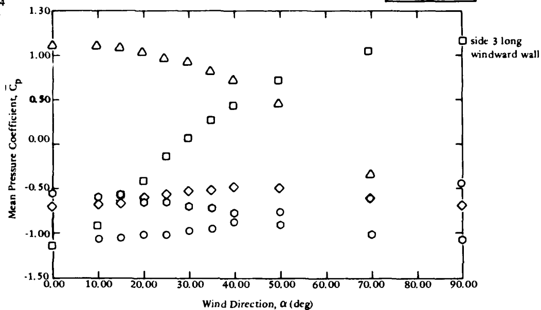
Figure C-7. Averaged local pressure coefficients, \bar{C}_p , for a side ratio of 0.25.
