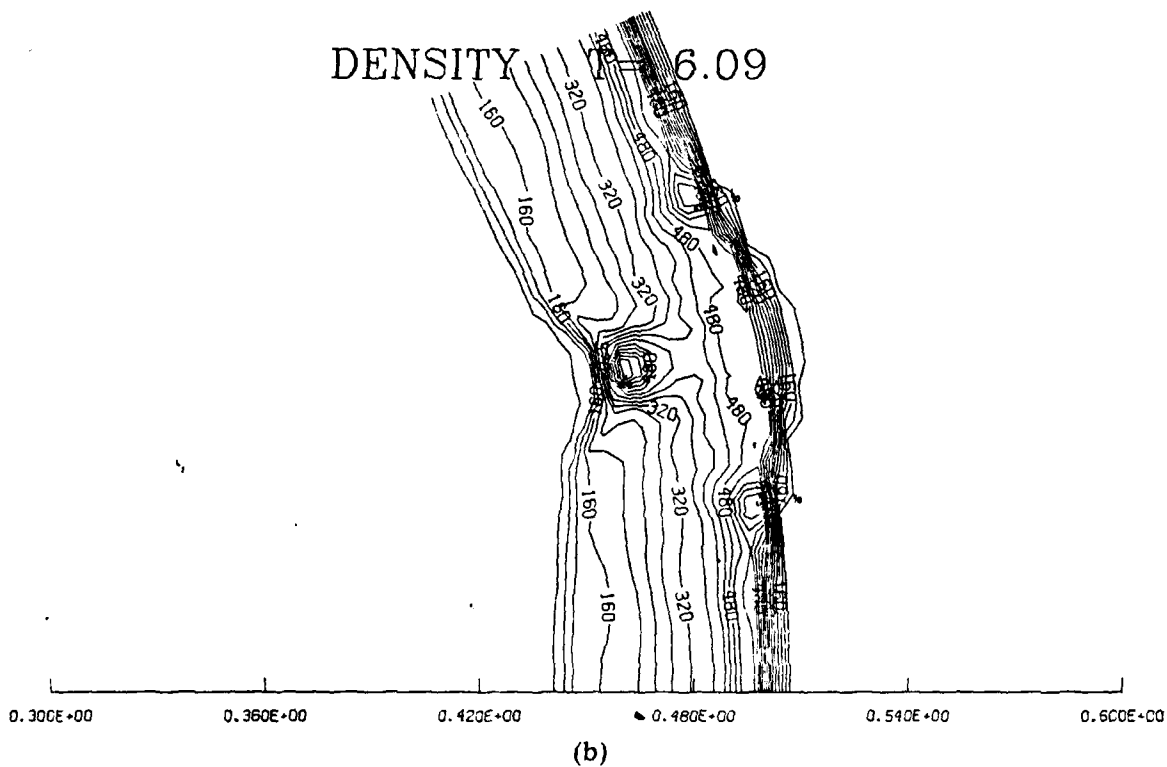
Fig. 4 — Density contours at selected times for a "large" jet type of perturbation. Display format is similar to Figure 1. Contours are labeled in units of 10^{-7} \text{ gm/cm}^3 . The times displayed are: 4.a = 2.6 ns, 4.b = 6.09 ns, 4.c = 13.39 ns, and 4.d = 41.4 ns.
