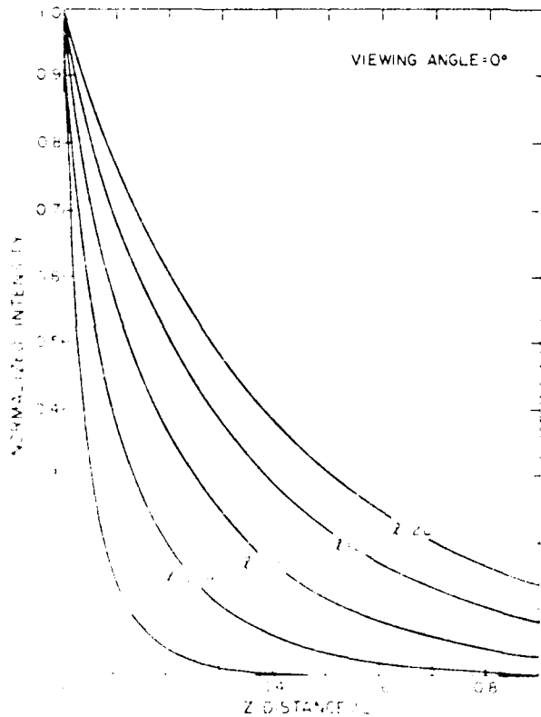
Fig. 4 Calculated line of sight intensity spatial distribution viewed from ahead for various choices of \lambda/L .
