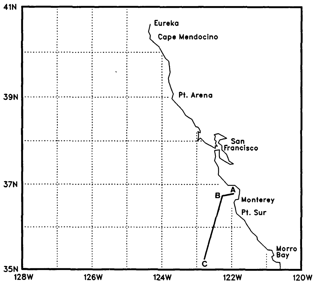
Figure 28: The cruise track for OPTOMA10.
