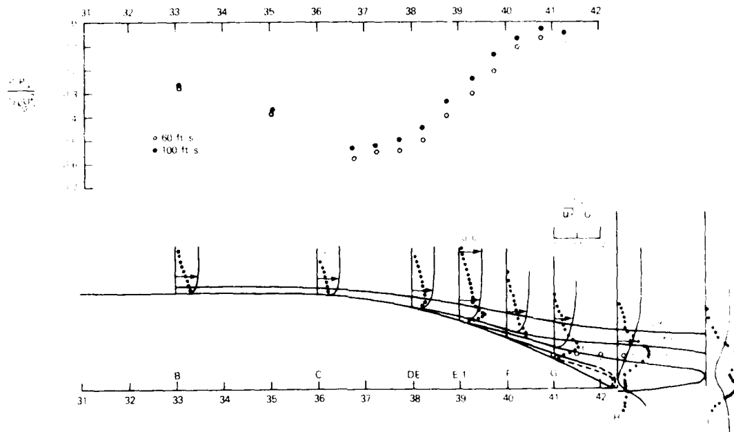
Figure 3 - Flow Patterns at U_\infty = 100 ft/s Pressure Distribution Near the 25^\circ Rounded Level
