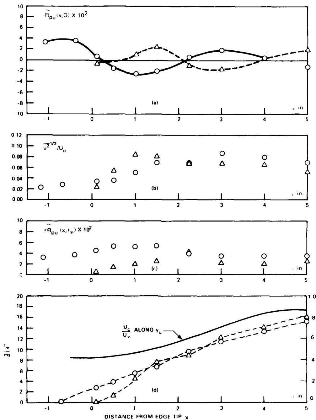
Figure 12 - Pressure-Velocity Correlations in the Wake Behind the 45° Rounded Beveled Edge at U_w = 50 ft/s; x Measured from the Lip. Points Marked 0 along y = y_u , \Delta along y = y_p . Velocity filtered in y_p -octave band at frequency f_s
