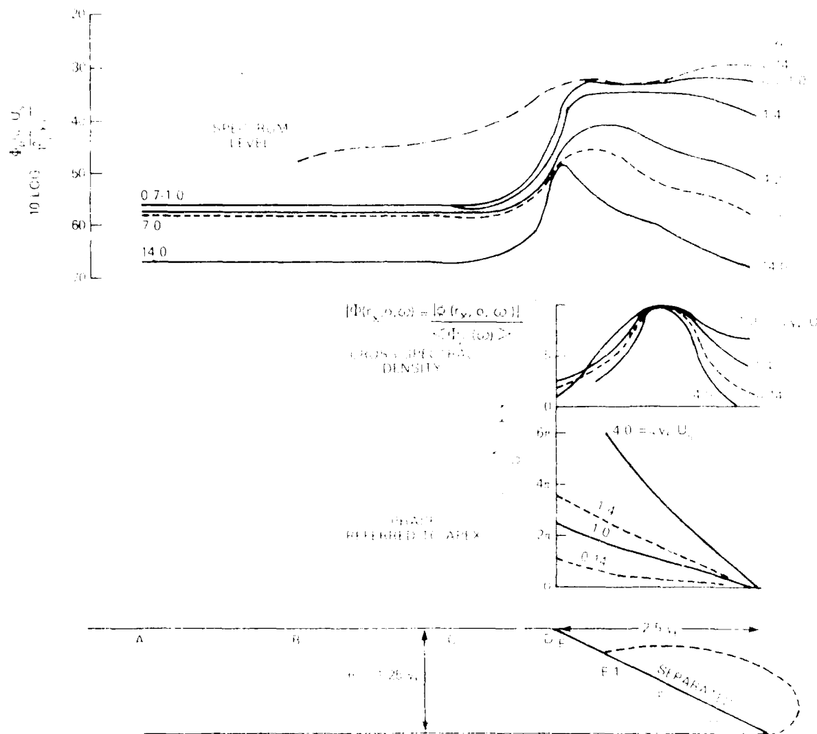
Figure 13 - Distribution and characteristics of pressures on the bench (cut in Figure 11) at x_1/U_\infty = 1.0 and U_\infty = 100 ft/sec.
