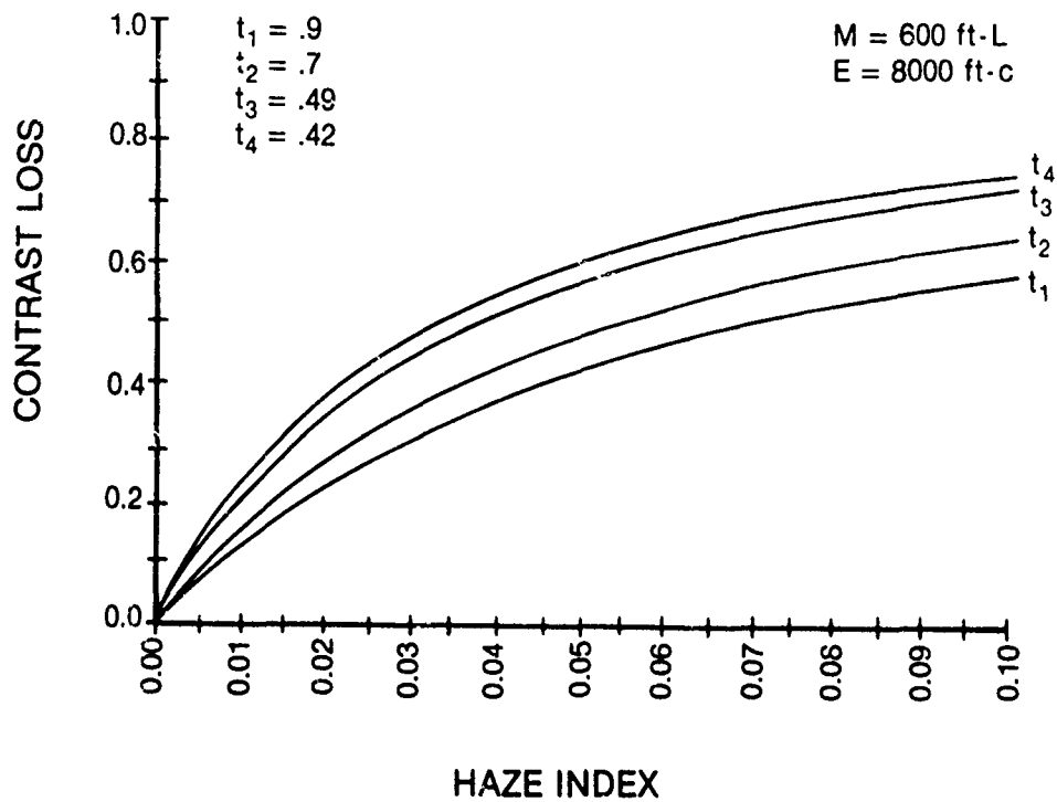
Figure 4. Contrast Loss for Different Transmissivities Versus Haze Index for a Sunny Day
