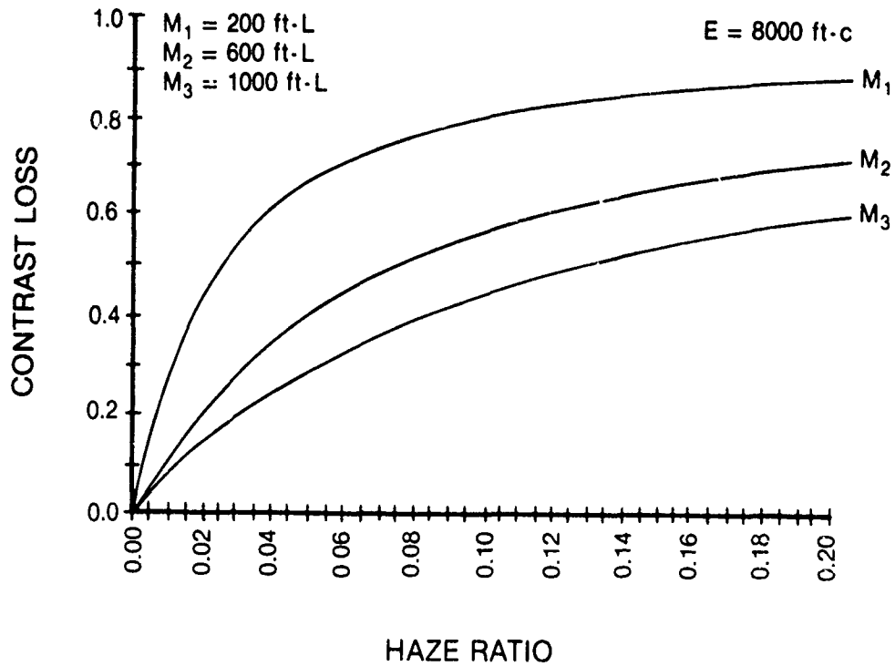
Figure 5. Contrast Loss Versus Haze Ratio for Bright Day Viewing Toward Sun
