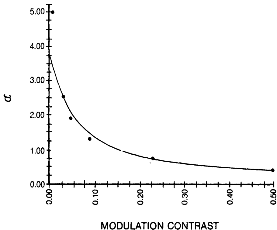
Figure 10, Angular Subtense at Detection versus Contrast for a Dark Circular Disk on a Light Background
