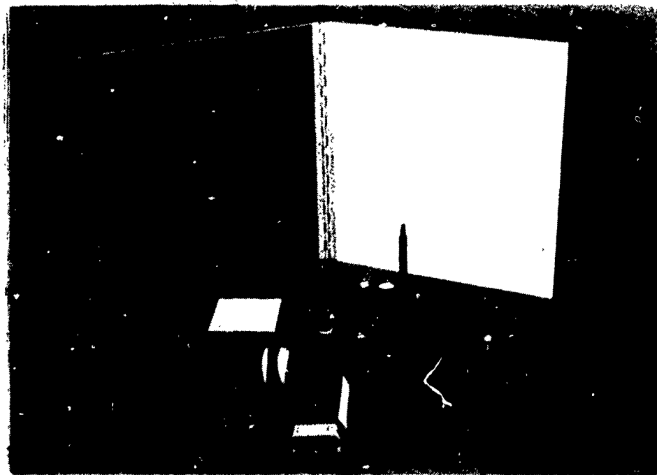
Figure 9. The Contrast Loss Measurement Kit
