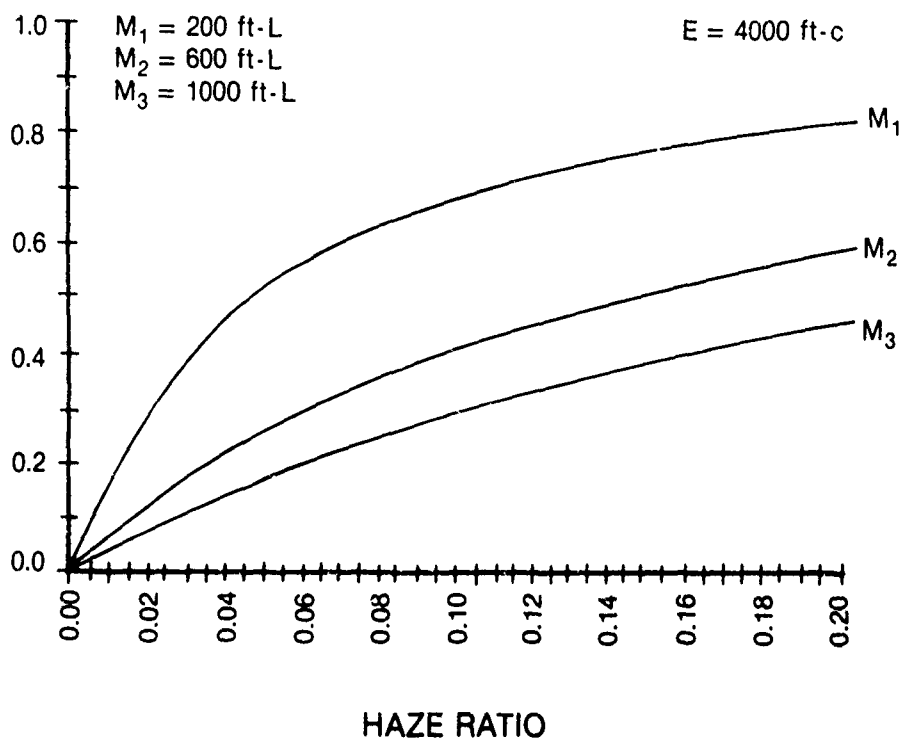
Figure 6. Contrast Loss Versus Haze Ratio for Bright Day Viewing at Moderate Angle From Sun
