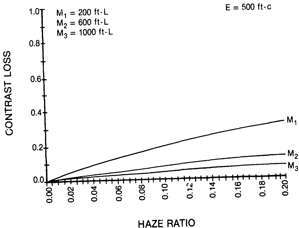
Figure 8. Contrast Loss Versus Haze Index for Bright Day Viewing Almost Directly Away from the Sun
