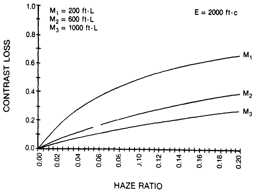
Figure 7. Contrast Loss Versus Haze Index for Bright Day Viewing at a Large Angle from the Sun
