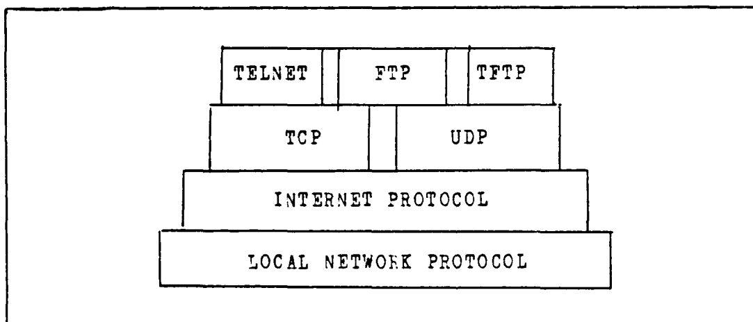
Figure 2.3 ARPANET Protocol Hierarchy
