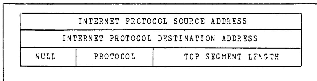
Figure 4.3 Pseudo Header Format
