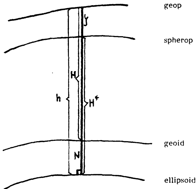
Figure 19. The Spatial Relationship Between Selected Gravimetric Quantities
