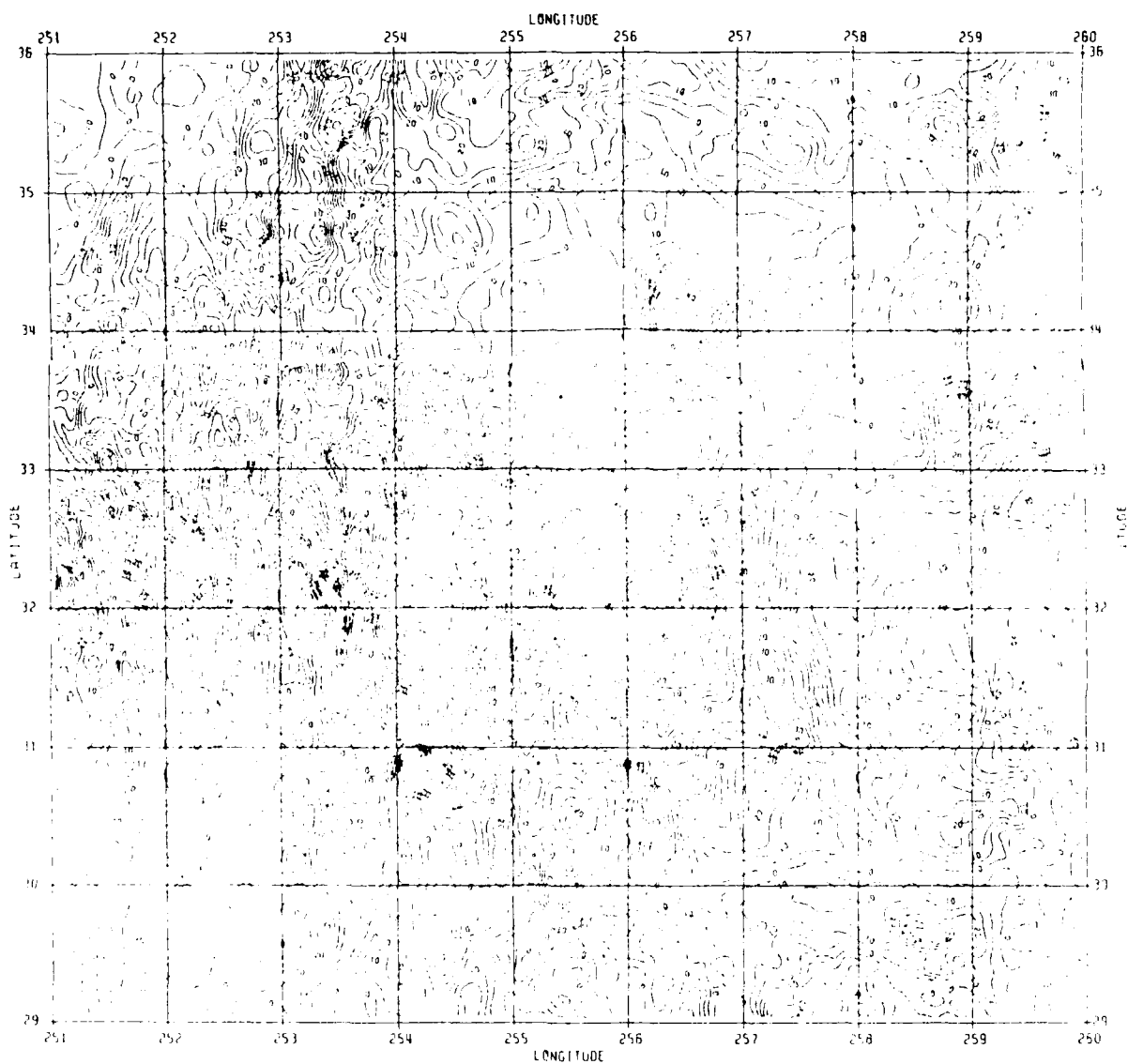
Figure 11. Residual Refined Bouguer Anomalies, New Mexico Balloon Gravity Test Site. C.I. = 5 mgals.
