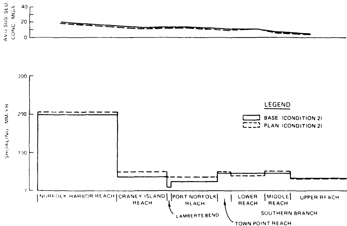
Figure 27. Elizabeth River, sedimentation results, base to plan (Flow 2)
