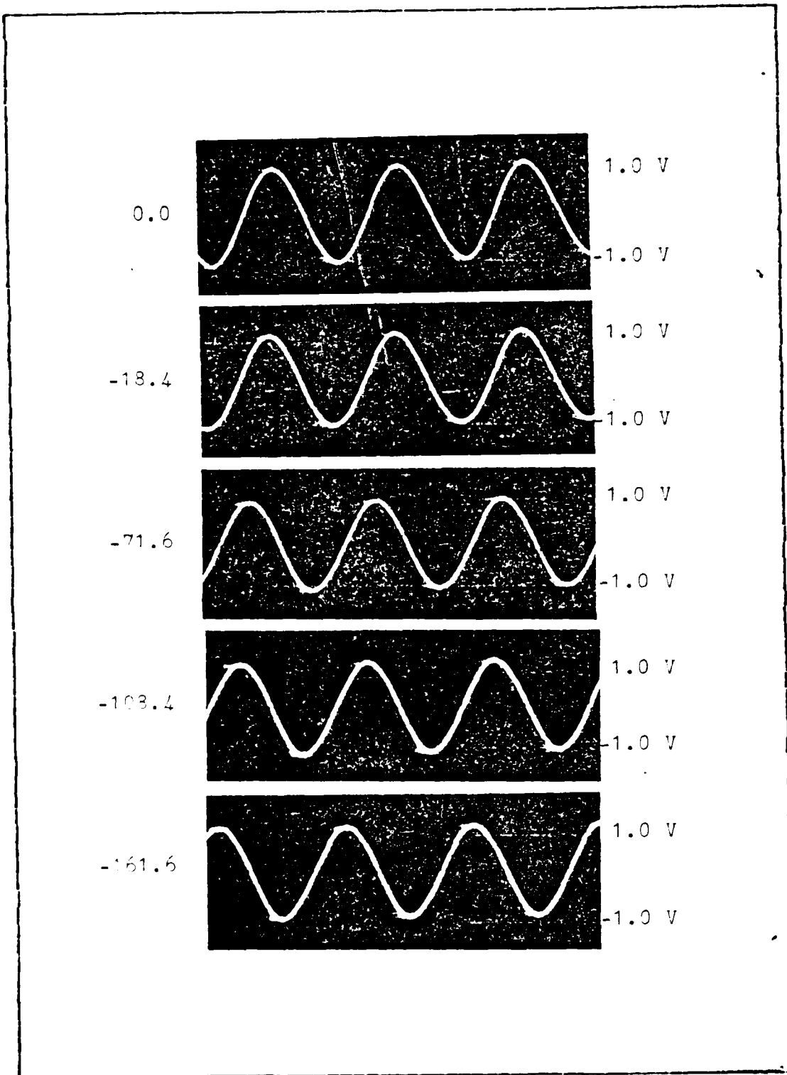
Figure 2.6 Photographs of Transmitter Output (Negative Phase)
