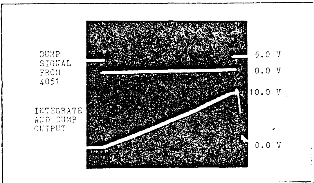
Figure 3.12 Photograph of Integrate and Dump
