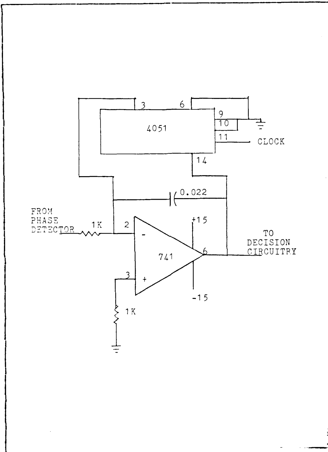
Figure 3.10 Circuit Diagram of Integrate and Dump
