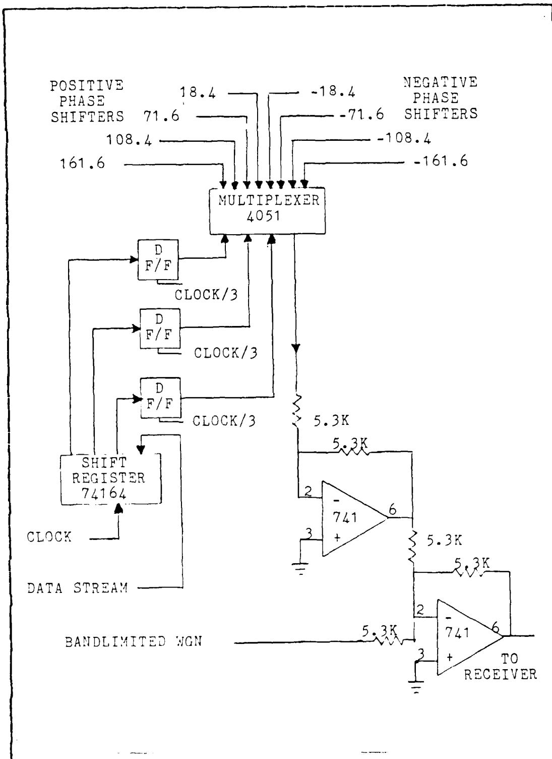
Figure 2.4 Circuit Diagram for Multiplexer, Inverter, & Summer
