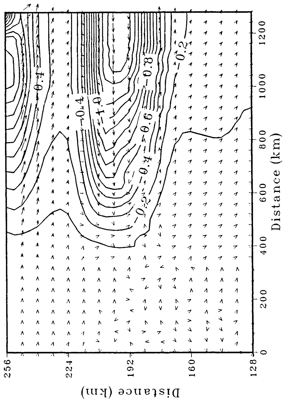
Figure 4-8. As in Fig. 4-2 except for Experiment 4-3, and the maximum departure is about 35 cm s -1 .
