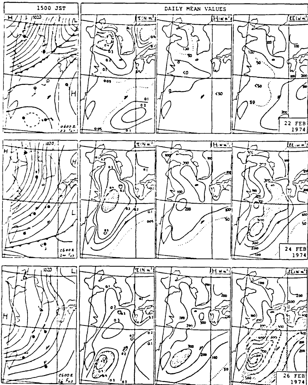
Figure 2-3. Surface pressure field and the daily mean distribution of the surface wind stress ( \text{N m}^{-2} ), sensible heat flux ( \text{W m}^{-2} ) and latent heat flux ( \text{W m}^{-2} ) during AMTEX 1974 (from Kondo, 1976). The top row is February 22, the middle row is February 24 and the bottom row is February 26.
