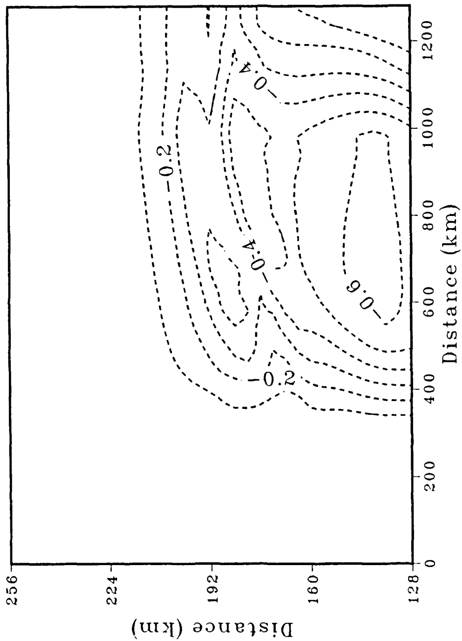
Figure 4-1. Surface v component at hour 72 for Experiment 4-1. Negative values indicate southward flow.
