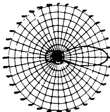
Directional antenna pattern.
