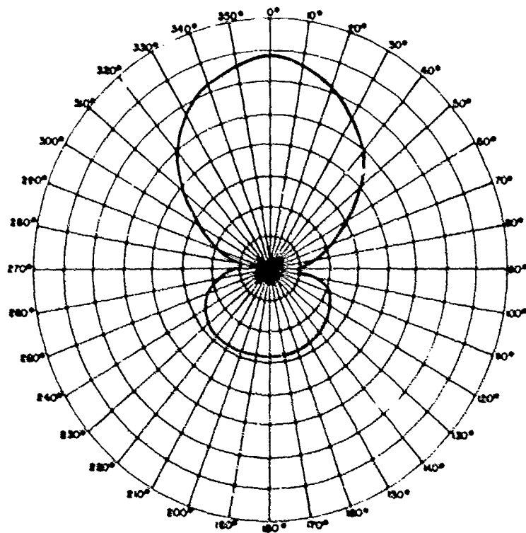
AS-2236 antenna azimuthal gain pattern, 76 MHz.
