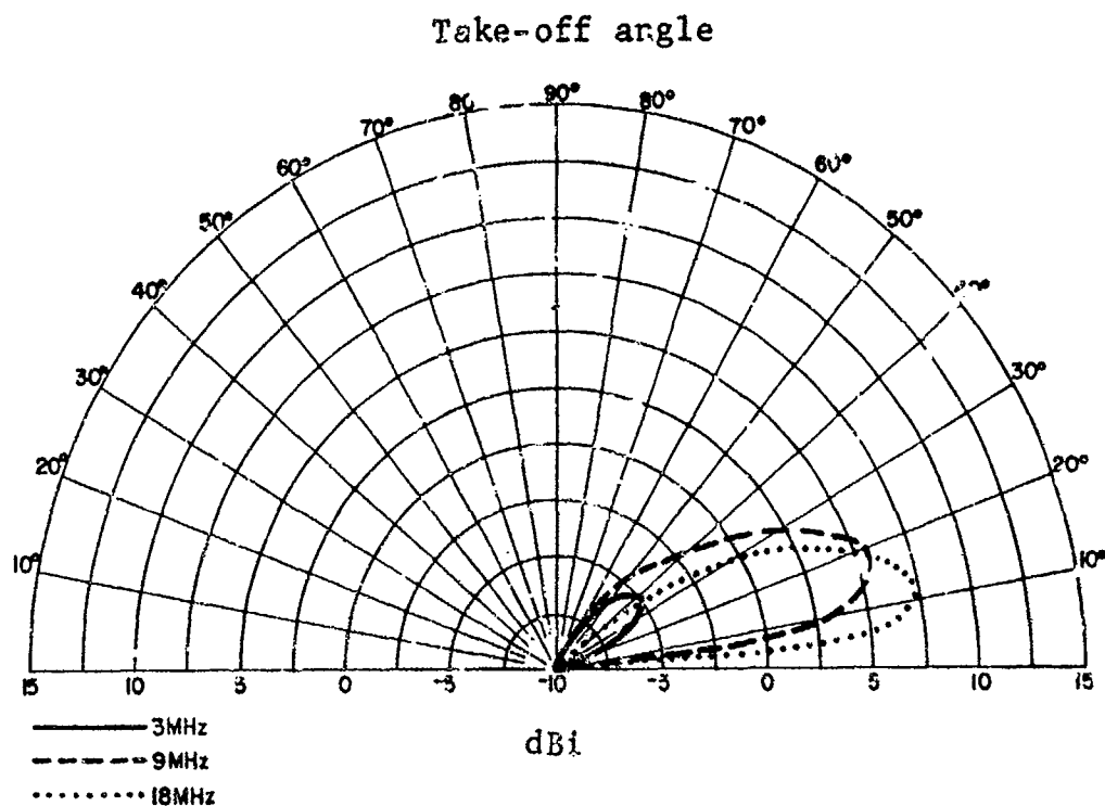
Terminated sloping vee antenna vertical pattern, height 40 feet, length 500 feet, apex angle 45°.
