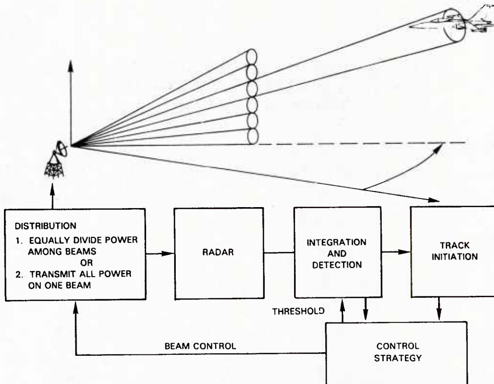
Fig. 1 — Representation of control strategy
