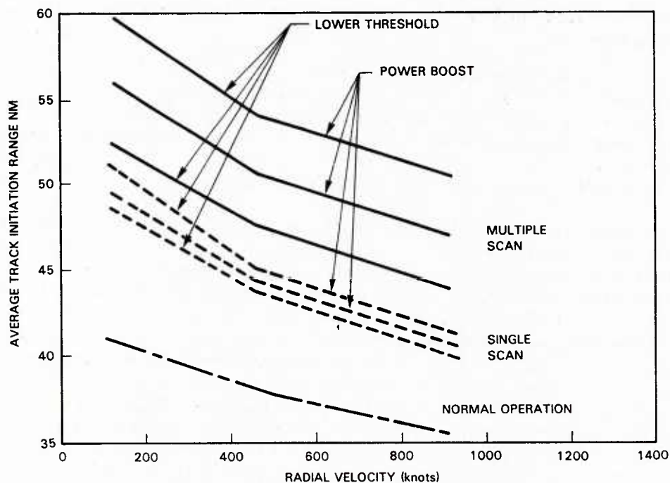
Fig. 3 — Average track initiation ranges versus radial velocity for a number of control strategies
