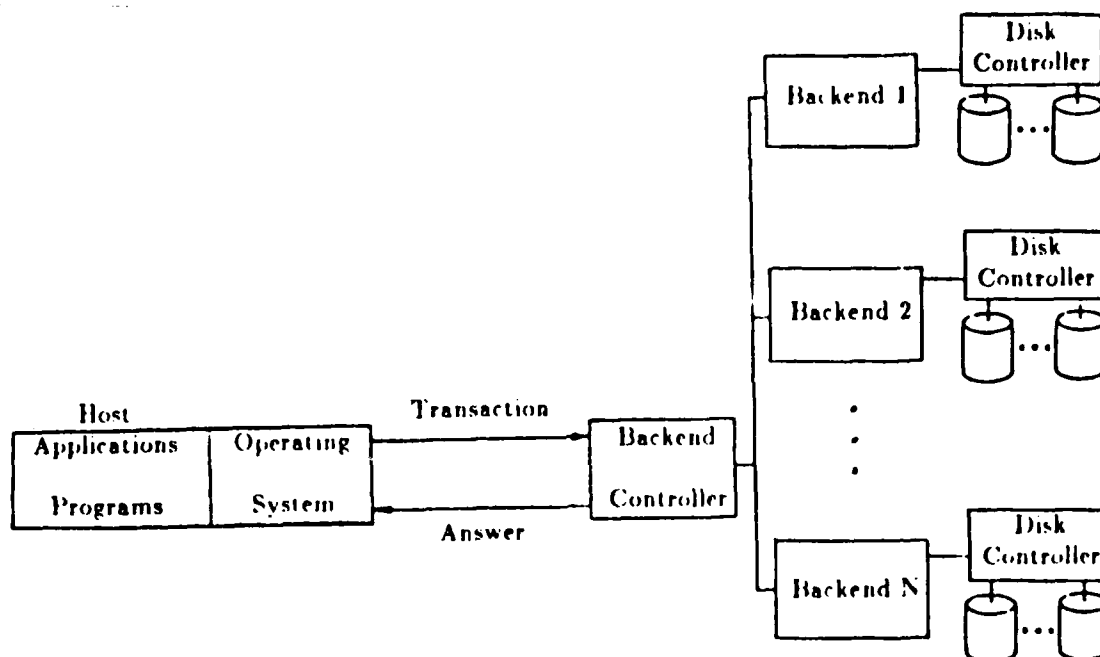
Figure 2. The Multi-Backend Database System (MBDS)
