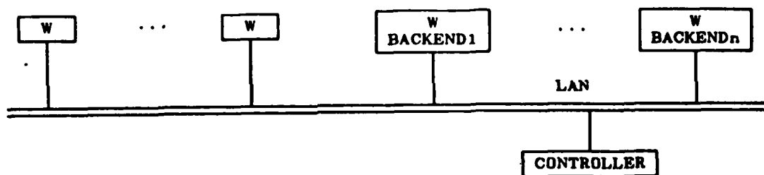
Figure 6. The Isolated-Controller Design
