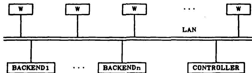
Figure 4. The Non-Integrated Single-LAN Design
