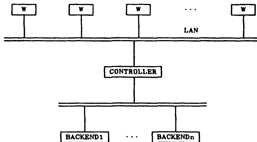
Figure 3. The Non-Integrated Dual-LAN Design
