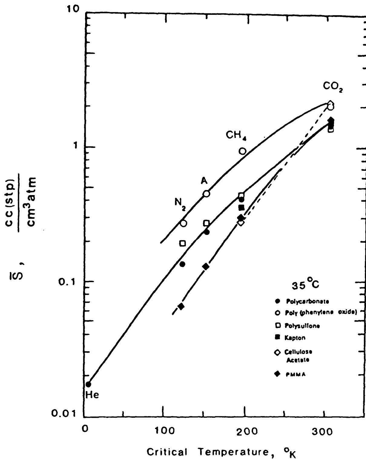
Figure 5: Correlation of the apparent solubility at 20 atm and 35°C with the critical temperatures of various penetrants in a number of glassy polymers.
