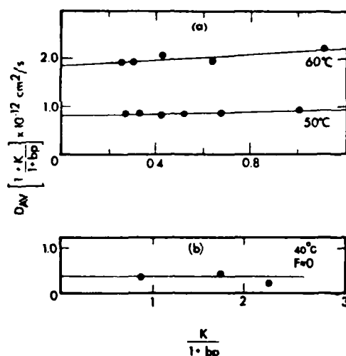
Fig. 8. Average diffusion coefficient values (see Table II) plotted according to eq. (15).
