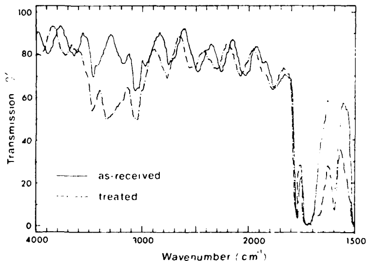
Figure 8. Infrared spectra of the as-received and the NH_3 exposed Kapton® samples. Note the increased absorbance in both the 1630-1700\text{ cm}^{-1} and 3200-3500\text{ cm}^{-1} regions, consistent with the postulated reaction between NH_3 and the imide structures.
