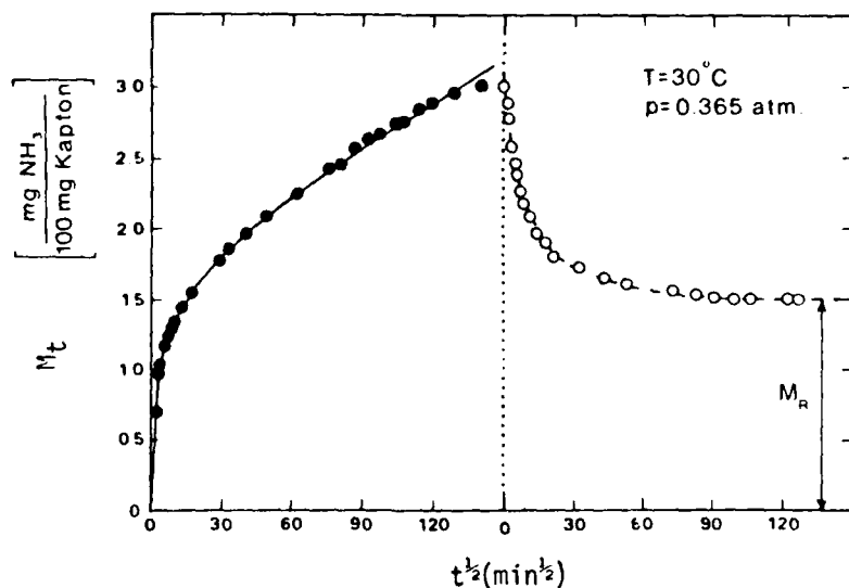
Figure 7. Sorption (●)/desorption (○) kinetic runs for a 0.5 mil Kapton® film at 30°C and at a NH 3 pressure of 0.365 atm. Note that at desorption equilibrium, 1.49 mg NH 3 /100 mg of Kapton® ( M_R ) remained in the polymer after protracted desorption under vacuum.
