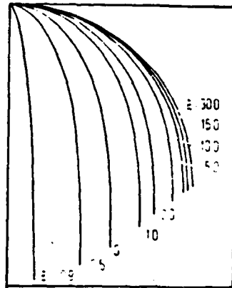
Figure 2.3 Adamek [27] Condensate Surface Profiles
