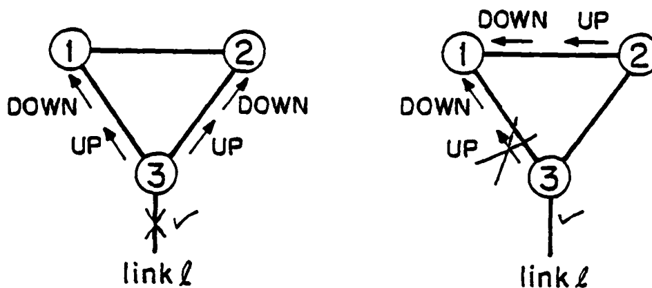
Figure 1.2.1: Topology Problem Example
