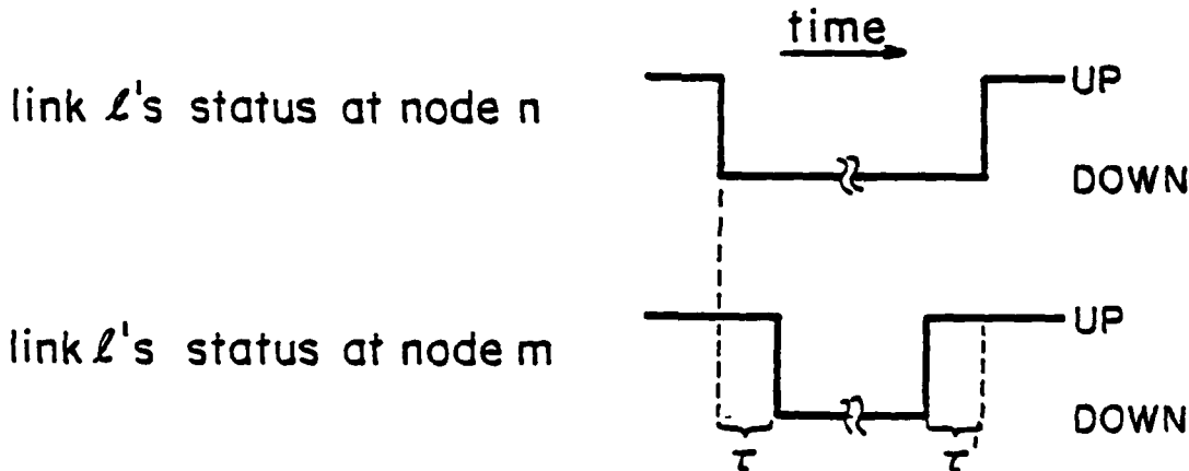
Figure 3.1.1: Ordinary DLC Status Change
