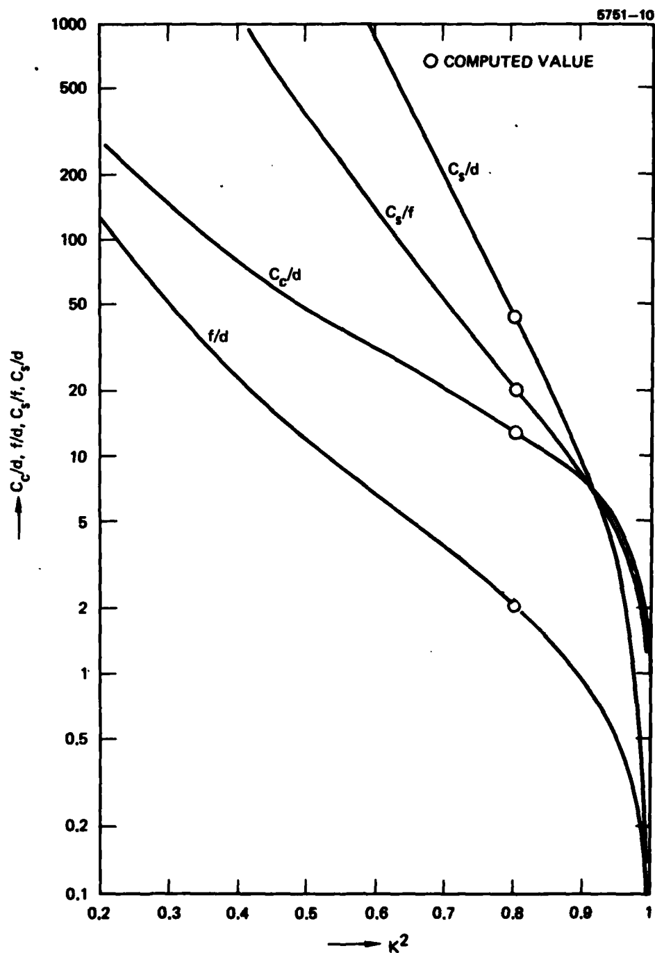
Figure III-3. Theoretical focal length and chromatic and spherical aberration constants for Glasser einzel lens along with computed values using Munros computer program.
