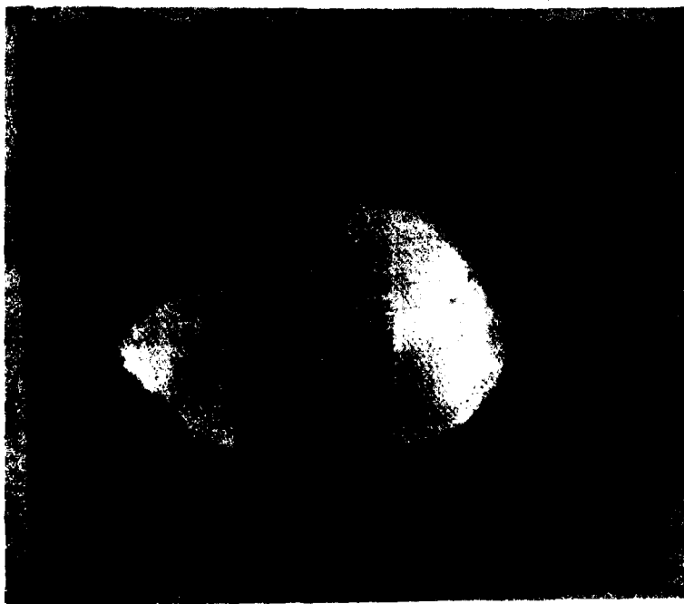
Figure B-52. F-178 BMI Resin Composite Firewall 114B-88 After Fire Penetration Test
