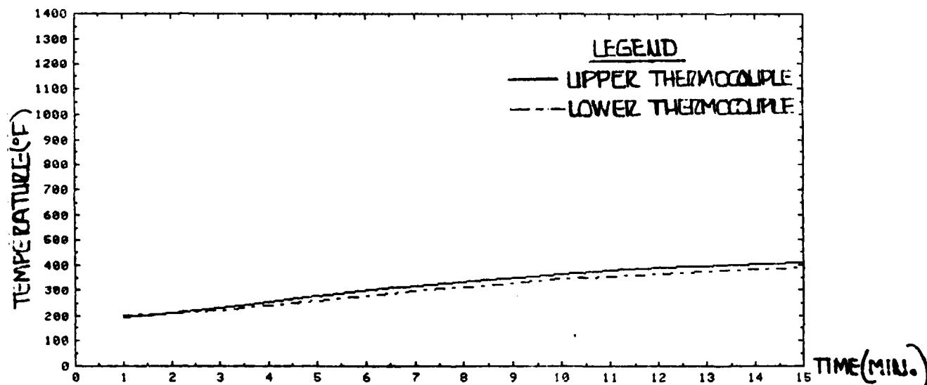
Figure 19. Non-Flame Side Temperature Profile of Flexible Min-K R HTS
