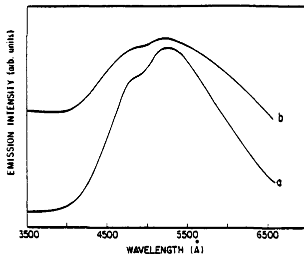
Fig. 13. Room temperature emission spectra of crystalline \text{Li}_2\text{WO}_4 powder. Excitation wavelength = (a) 2700 Å, (b) 2850 Å.
