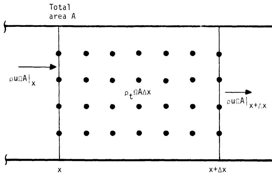
Figure 2-3 Stationary control volume for determination of the conservation of mass relation for porous materials
