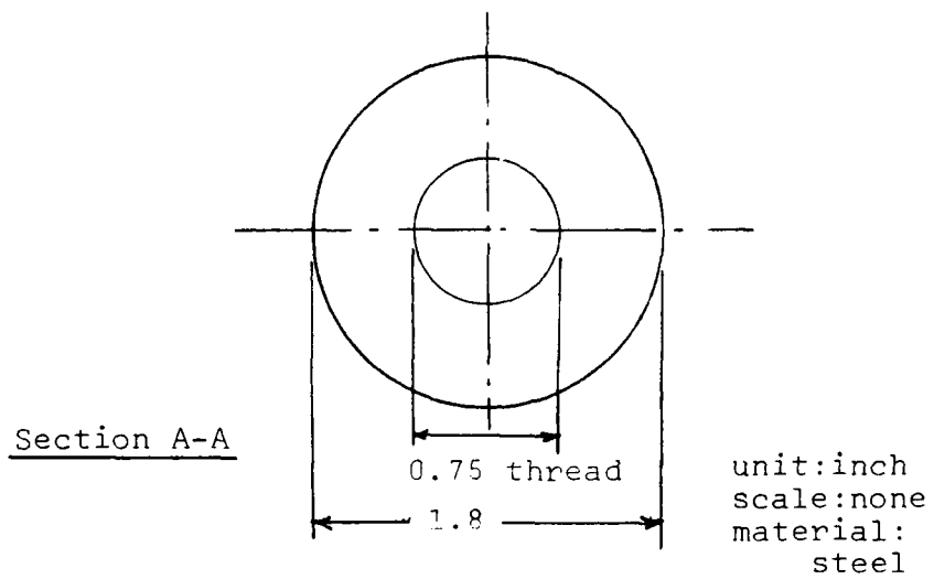
Figure D.2. New Design Wedge Coupling System:
