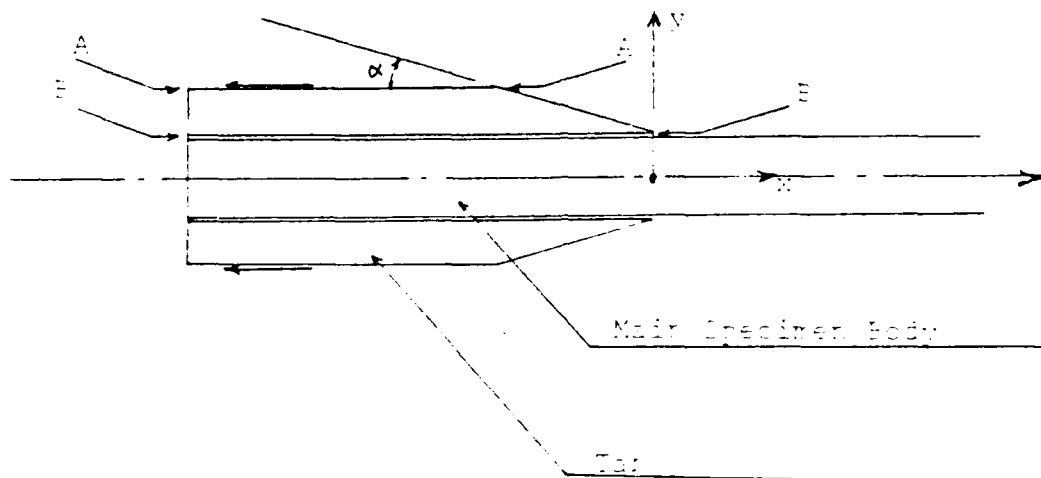
Figure 4.5. Stresses in Tab Region
