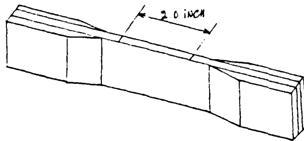
Figure 5.3. Gauge Mark
