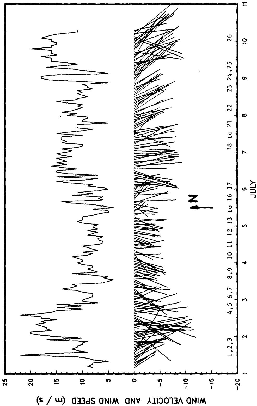
Figure 10 : Time-series of hourly true wind speed with true wind velocity sticks below the curve to indicate direction (North is given by the arrow). The time axis is annotated with the radioisotope launch numbers at their approximate launch times (OPTOMALL, Leg DII).
