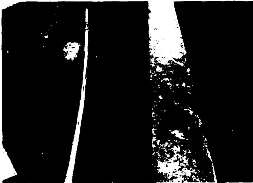
Photo No. 9 - Subsidence of fill along dam crest at water works inlet structure (STA. 2+70).
