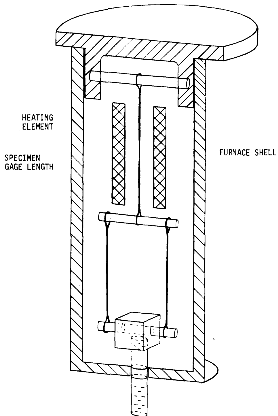
Figure 16. Furnace load path for axial creep and rupture specimens
