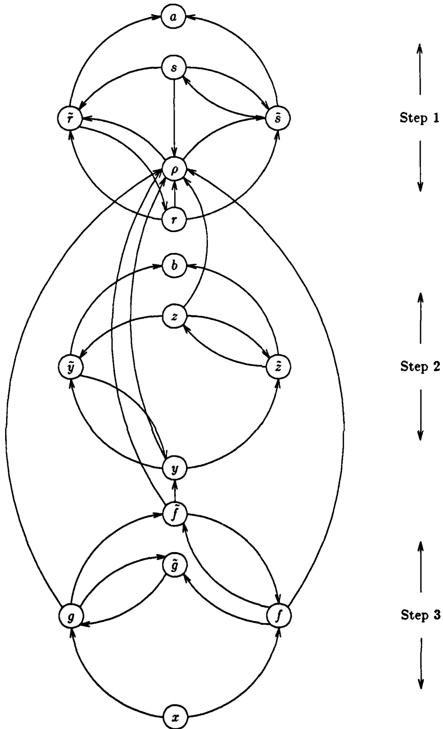
Figure 1: Dependence Graph for Steps 1, 2 and 3.
