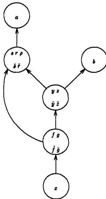
Figure 2: Acyclic Graph Obtained from the Directed Cut-Sets of the Dependence Graph.
